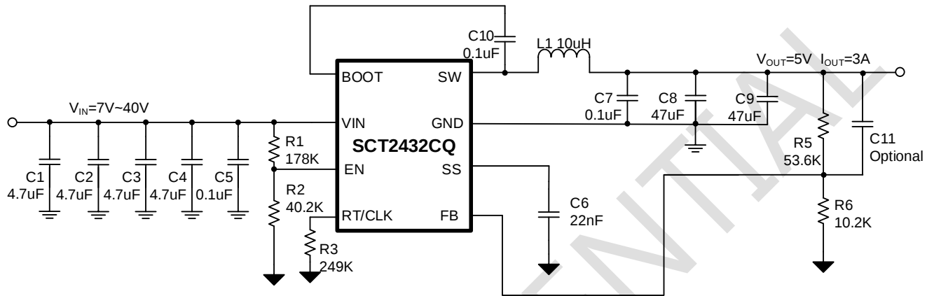
Figure 11. SCT2432CQ Design Example, 5V Output with Programmable UVLO
