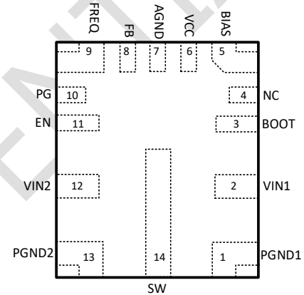
Figure1. 14-Lead FCQFN 4mmx4mm (Sketch Map)
