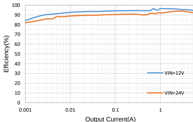
Efficiency, V OUT =5V, F sw =400KHz
