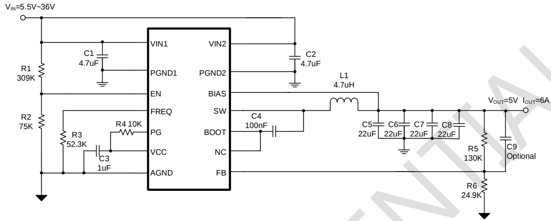
Figure 12. SCT2461MQ Design Example, 5V Output with Adjustable UVLO
