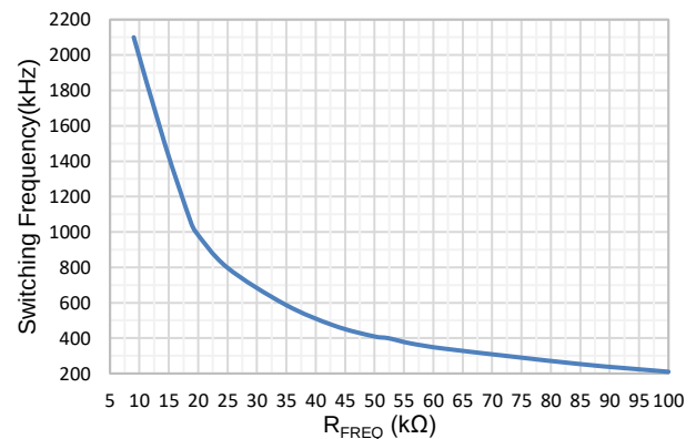
Figure 7. Clock Frequency vs FREQ Resistor
