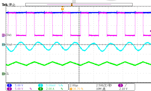
Figure 22. Output Ripple ( I_{LOAD}=2A )
