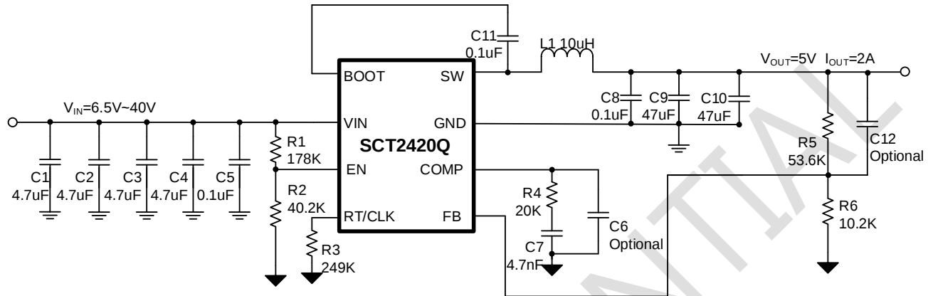
Figure 11. SCT2420Q Design Example, 5V Output with Programmable UVLO
