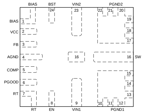
Figure 1. 24-Lead FCQFN 4mm×4mm
