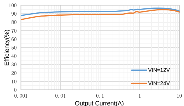
Efficiency, F_{sw}=400kHz , BIAS= V_{OUT}=5V
