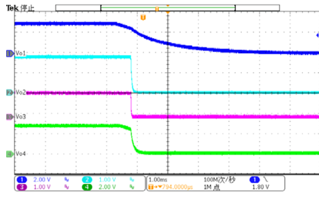
Figure 16. Power Off ( I_{o2}=0.6A , I_{o3}=1.2A , I_{o4}=0.3A )
