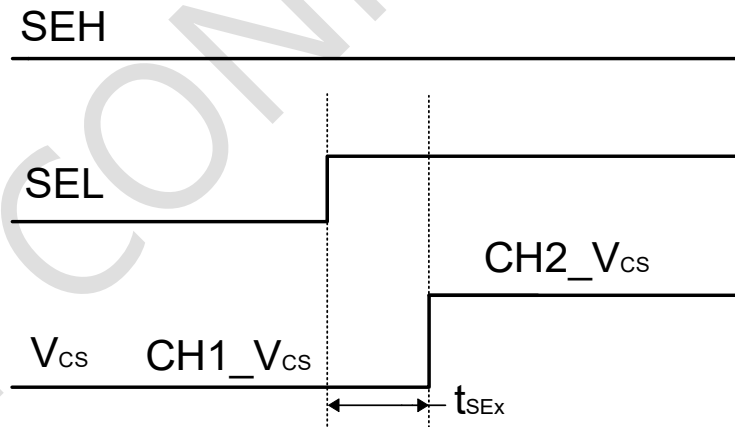
Figure 3. Multi-Sense Transition Delay
