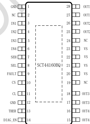
Top View: Version B ETSSOP-28
