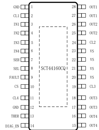
Top View: Version C ETSSOP-28
