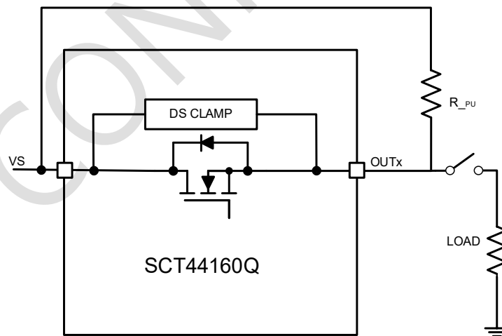
Figure 12. Open-Load Detection
