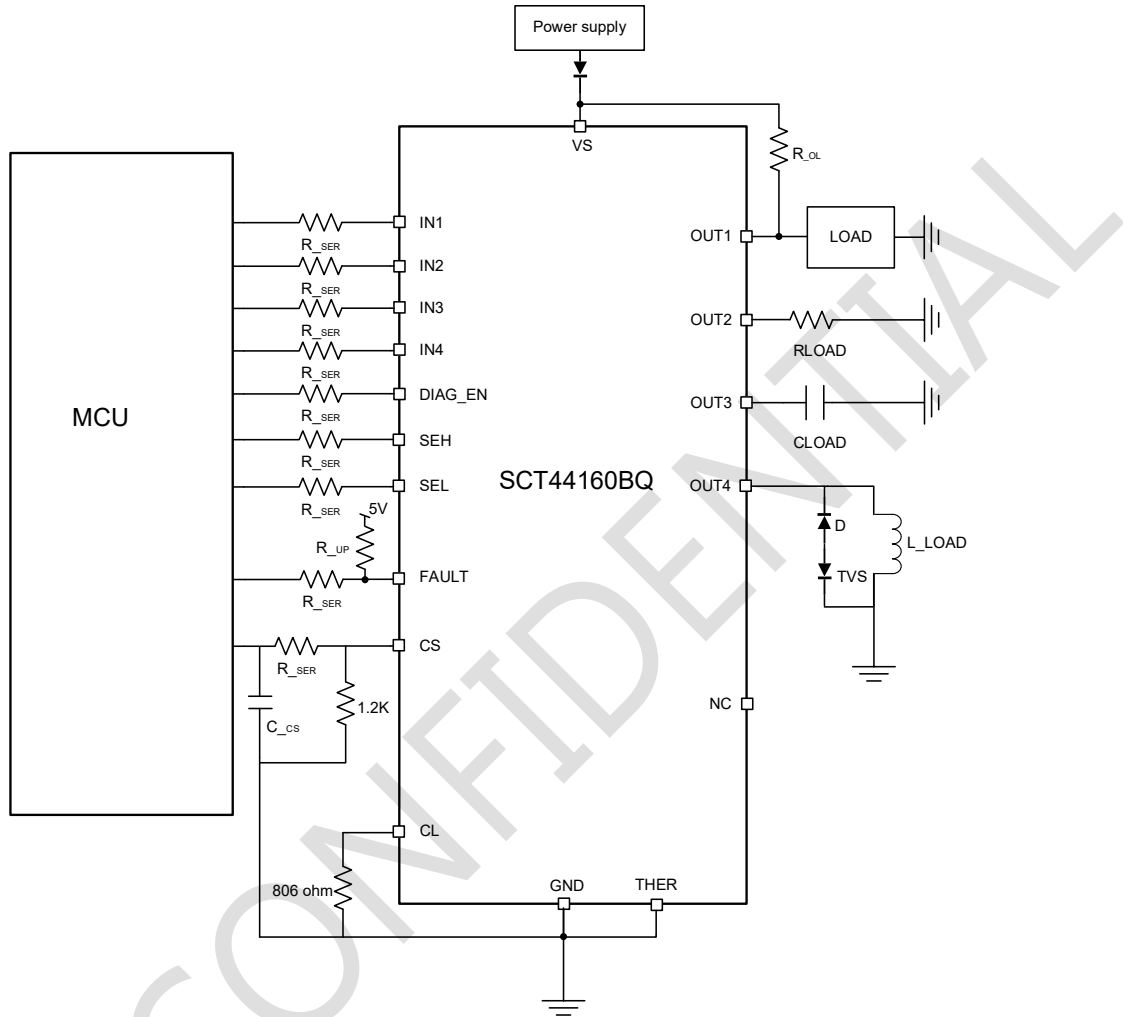
Figure 20. Version B Application Schematic
