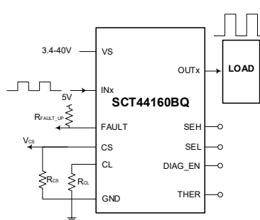
Typical Application of Version B
