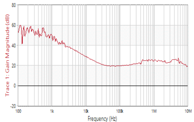
LDO PSRR, V_{OUT4}=2.8V , I_{OUT4}=100mA
