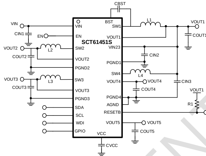
SCT61451S Radar PMIC Typical Application Circuit
