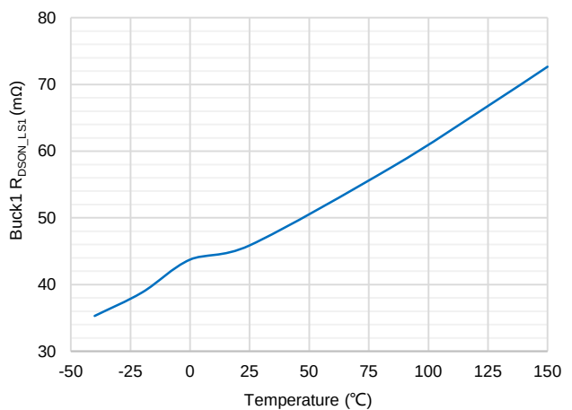
Buck1 R_{DS(on)_LS1} vs. Temperature
