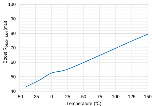
Boost R DS(on)_LS4 vs. Temperature
