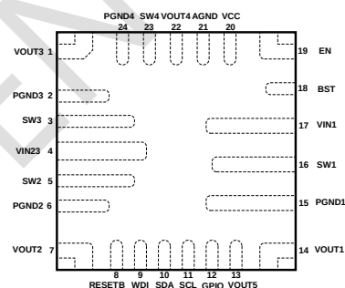
Top View: 24-Lead FCTQFN 4mmx4mm
