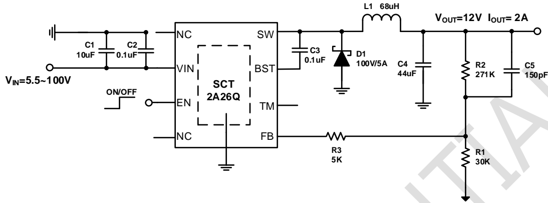
Figure 10. SCT2A26Q Design Example, 12V Output with Programmable UVLO
