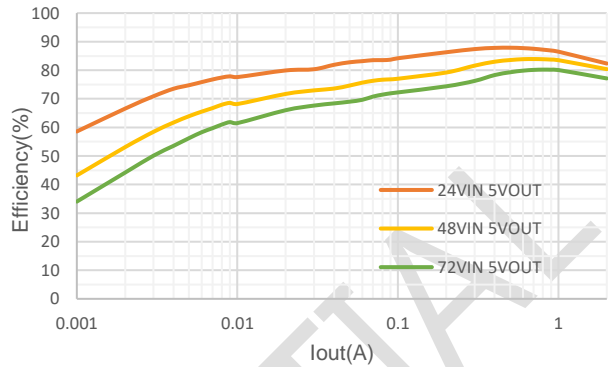
Figure 3. Efficiency vs Load Current, Vout=5V
