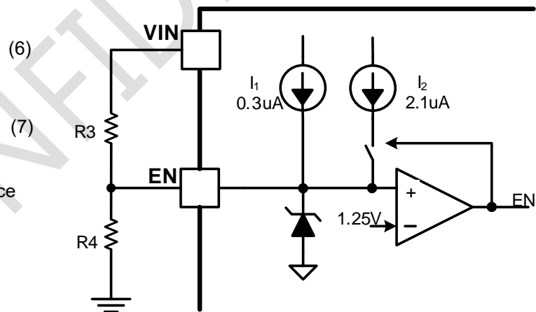
Figure 11. System UVLO by enable divide
