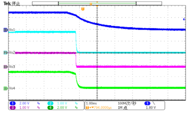
Figure 16. Power Off ( I_{o2}=0.6A , I_{o3}=1.2A , I_{o4}=0.3A )
