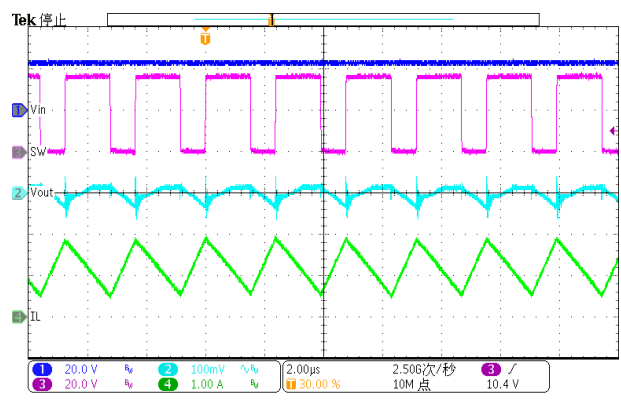
Figure 32. Steady-state (Iload=2A)
