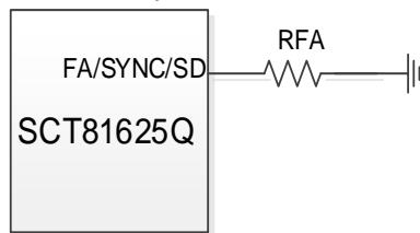
Figure14. Frequency Adjust
