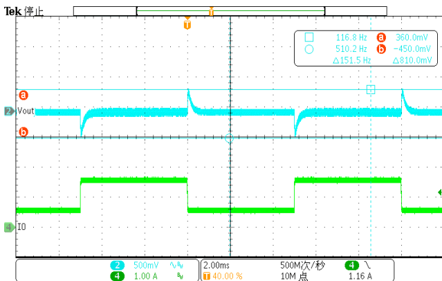
Figure 31. Load Trans (Iload=0.5A-1.5A)
