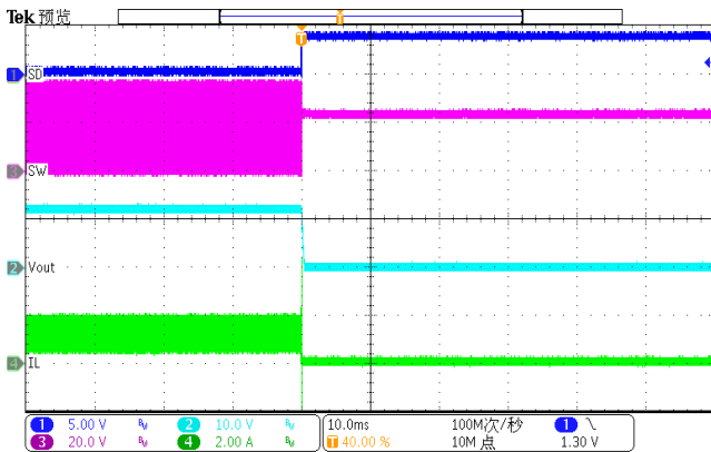
Figure 29. Shutdown remove
