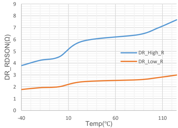
Figure 10. DR Resistance vs Temperature
