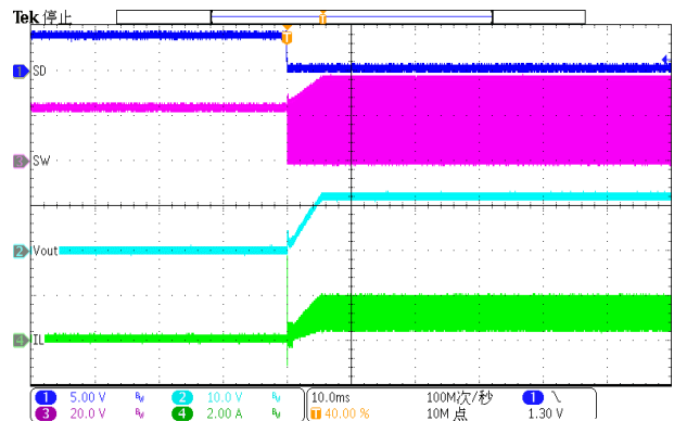
Figure 30. Shutdown remove
