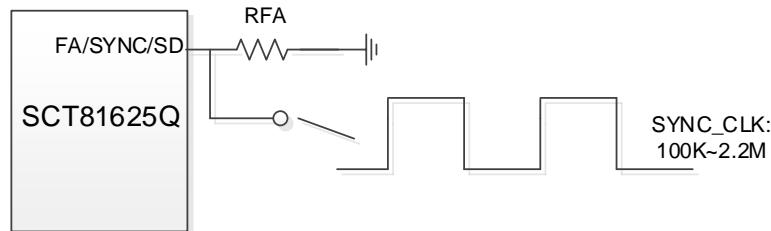
Figure15. Frequency Sync
