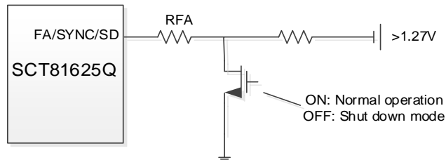
Figure16. Shutdown operation in Frequency Adjust Mode
