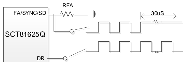
Figure17. Shutdown operation in Frequency Synchronization Mode
