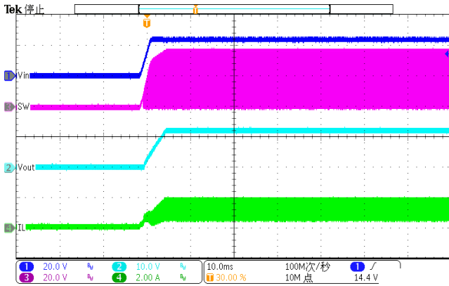
Figure 27. Power up(Iload=2A)
