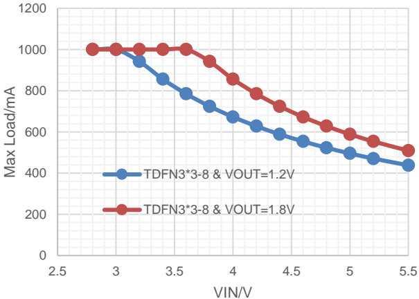
Figure 27. Maximum Output Current vs Input Voltage, DFN3X3-8L,TJ ≤ 125°C
