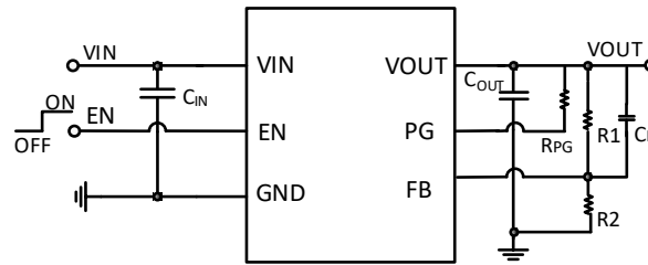
Figure 21. SCT71010A00 Typical Application Schematic
