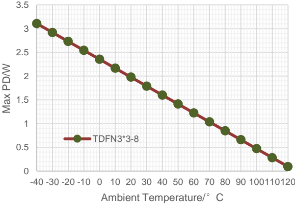
Figure 28. Maximum Allowed Power Dissipation vs Ambient Temperature, DFN3X3-8L,TJ ≤ 125°C
