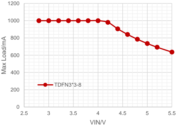
Figure 26. Maximum Output Current vs Input Voltage, VOUT=1.8V of DFN3X3-8L ,TJ ≤ TSD_R
