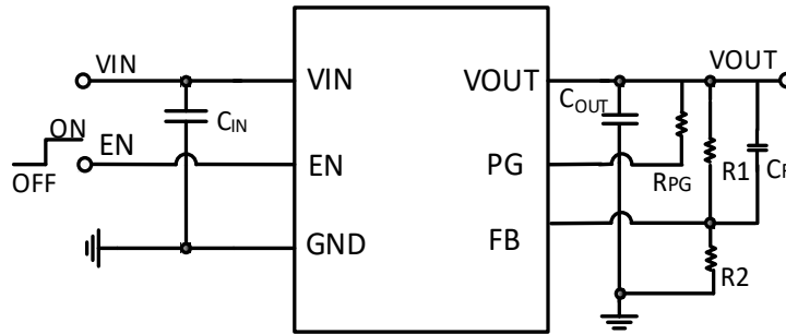
Figure 22. SCT71005Q Typical Application Schematic
