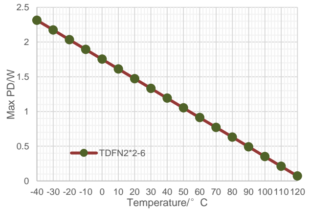
Figure 30. Maximum Allowed Power Dissipation vs Ambient Temperature, DFN2X2-6L, T_J \leq 125^\circ\text{C}
