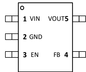
SCT71005A03QTWDR SOT23-5L Package
