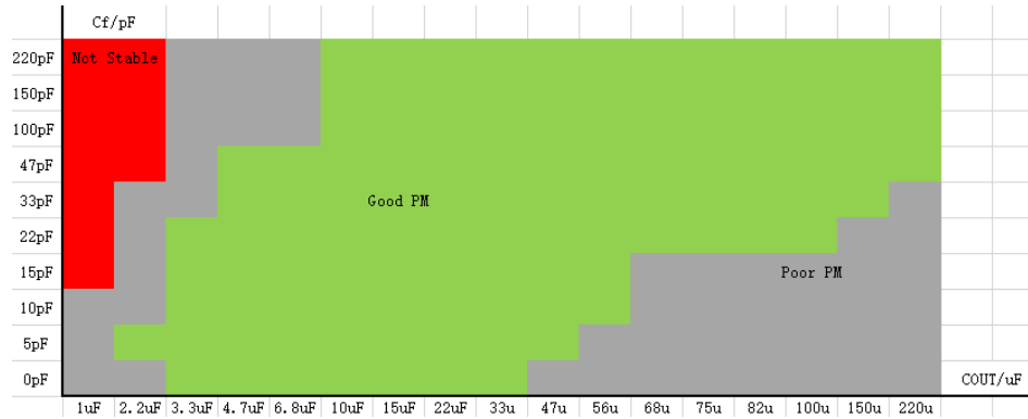
Figure 26. SCT71005Q Feed Forward Capacitors recommend( R_2=100k\Omega , V_{OUT}=1.8V )
