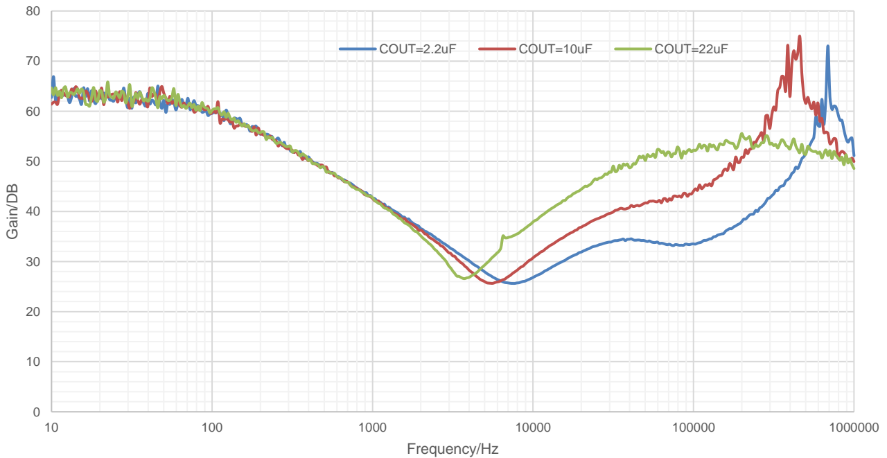
Figure 12. PSRR vs Frequency VIN=3.3V,VOUT=1.2V,Cf=33pF,IOU=10mA
