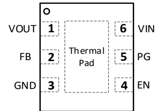
SCT71005A04QDVAR DFN2X2-6L Package
