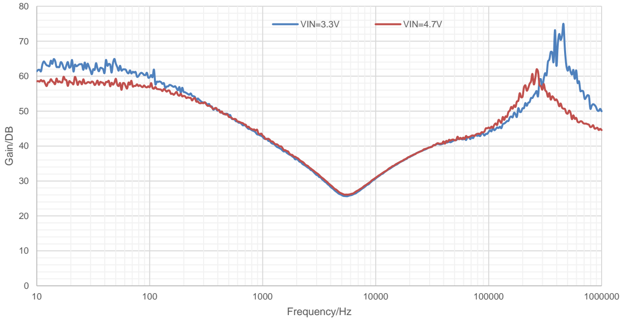
Figure 11. PSRR vs Frequency VOUT=1.2V,Cf=33pF,COU=10uF,IOU=10mA
