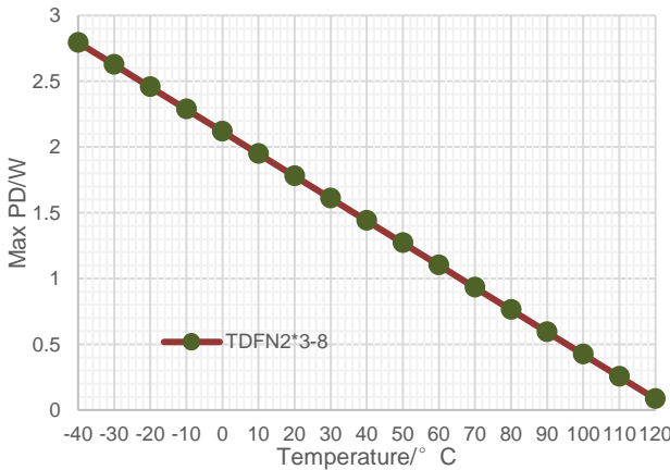
Figure 31. Maximum Allowed Power Dissipation vs Ambient Temperature, DFN2X3-8L, T_J \leq 125^\circ\text{C}
