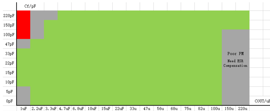
Figure 27. SCT71005Q Feed Forward Capacitors recommend( R_2=10k\Omega , V_{OUT}=1.8V )
