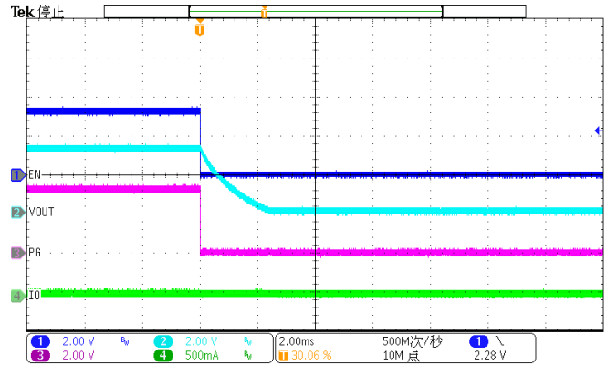
Figure 40. Disable (Iload=10mA)
