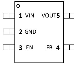
SCT71005A01QTWDR SOT23-5L Package
