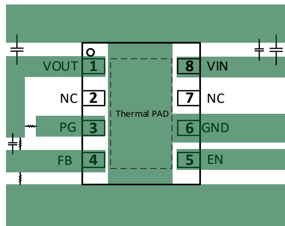
Figure 48. PCB Layout Example
