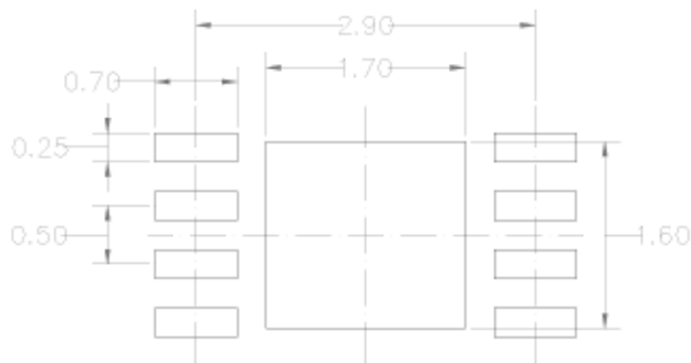
DFN2X3-8L Package Outline Dimensions
