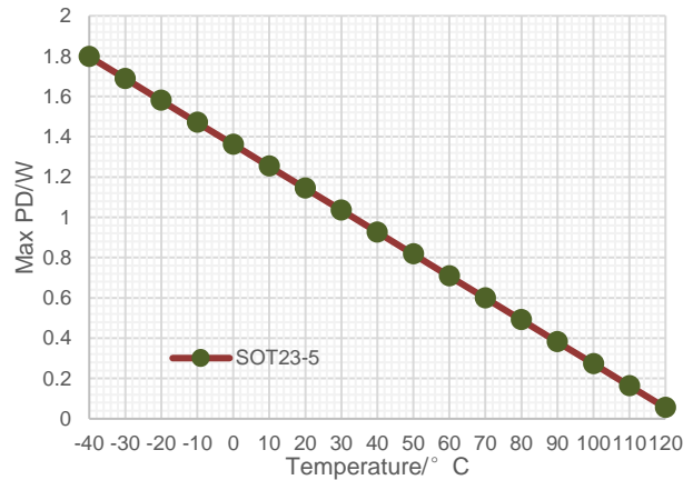
Figure 32. Maximum Allowed Power Dissipation vs Ambient Temperature, SOT23-5L, T_J \leq 125^\circ\text{C}
