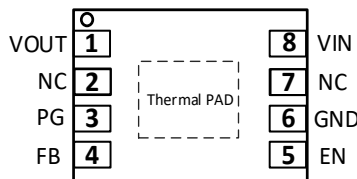
SCT71005A02QDTR DFN2X3-8L Package
