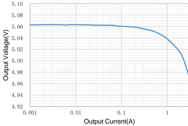
Figure 4. Load Regulation ( V_{in}=12V , V_{out}=5V )
