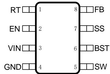
Figure 1. 8-Lead FCSOT583
