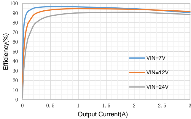
Figure 2. Efficiency, F_{sw}=500kHz , V_{out}=5V
