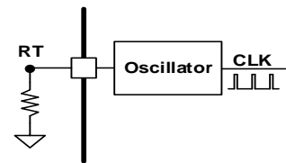
Figure 10. Setting Frequency and Clock Synchronization
