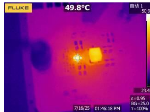
Figure 24. Thermal, 12Vin, 5Vout, 4A
