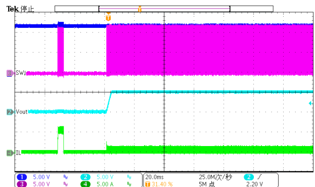
Figure 18. Over Current Release (hard short to 0.1A)
