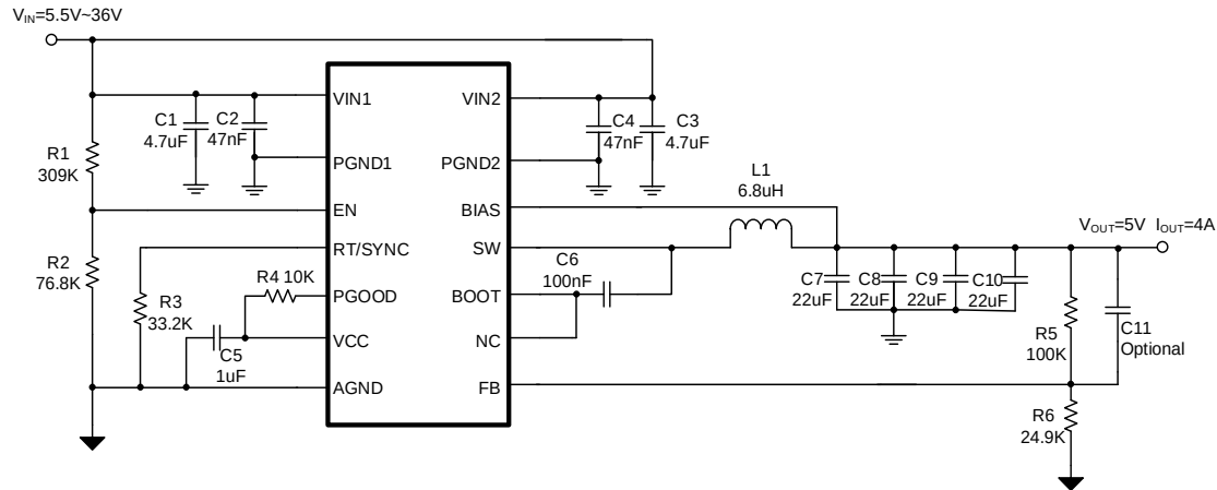
Figure 12. SCT2444 Design Example, 5V Output with Adjustable UVLO
