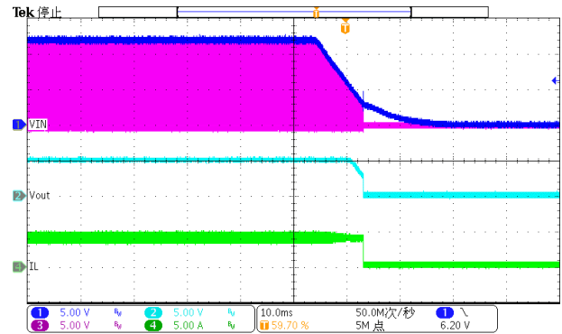
Figure 14. Power down (Iload=4A)
