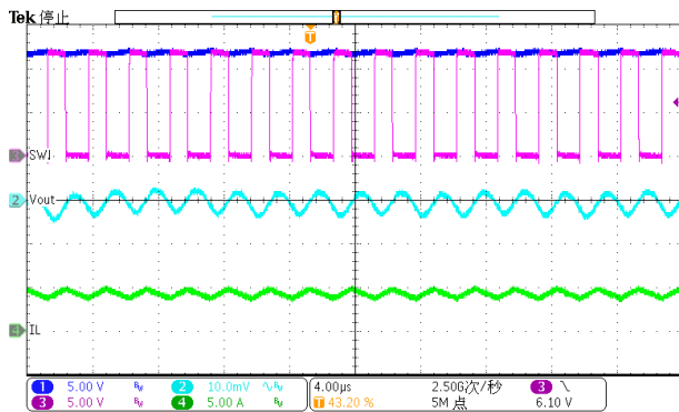
Figure 23. Output Ripple (Iload=4A)
