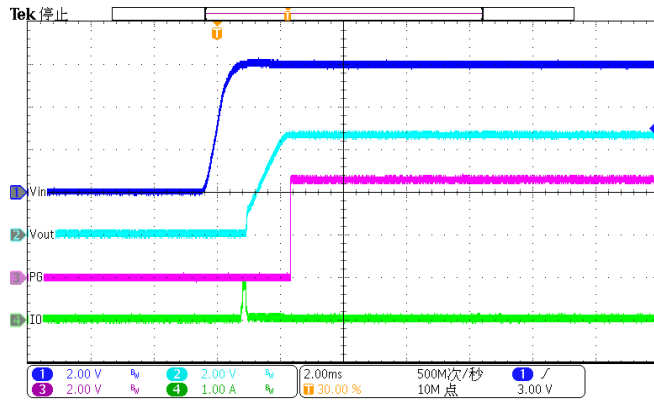
Figure 35. Power up (Iload=10mA)
