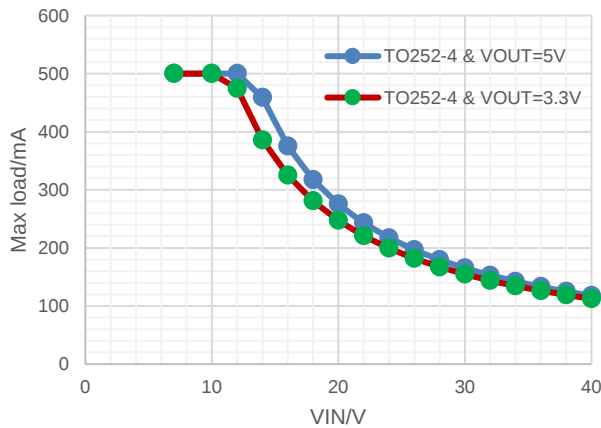
Figure 33. Maximum Output Current vs Input Voltage, TO252-4L, T_J \leq 125^\circ\text{C} (4-layer EVM)
