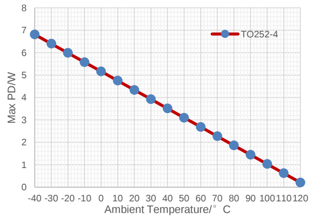
Figure 34. Maximum Allowed Power Dissipation vs Ambient Temperature, TO252-4L, T_J \leq 125^\circ\text{C} (4-layer EVM)
