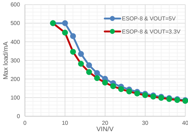
Figure 31. Maximum Output Current vs Input Voltage, ESOP-8L, T_J \leq 125^\circ\text{C} (4-layer EVM)
