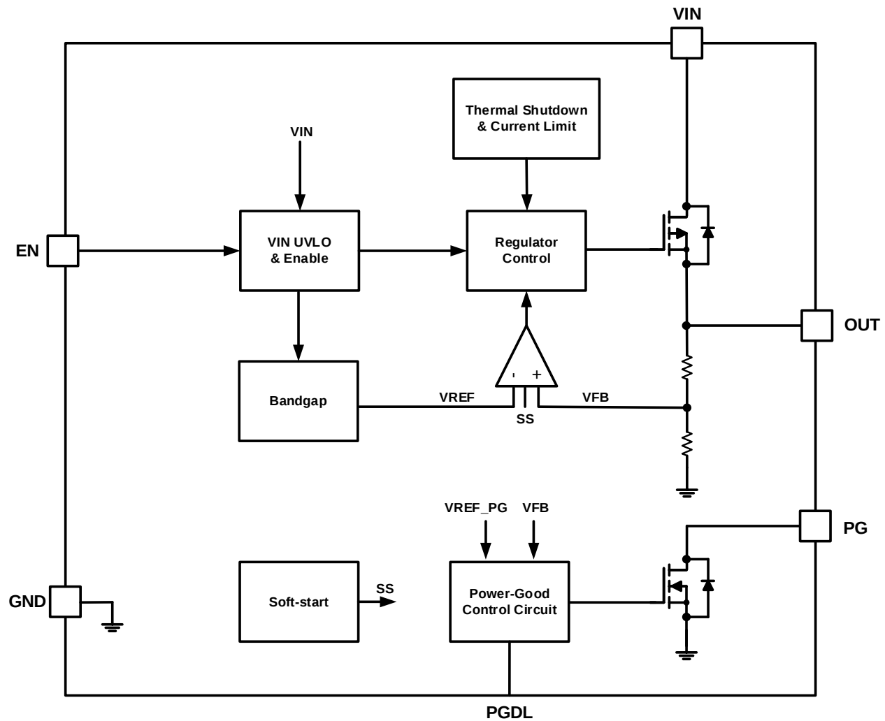
Figure 17. Fixed Output Version Functional Block Diagram
