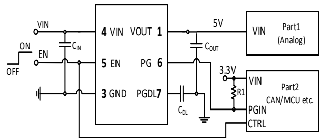
Figure 23. PG Connected to the other Power Supply
