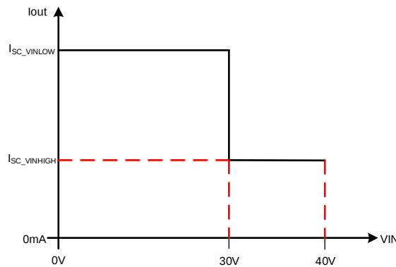
Figure 20. Current Limit with Foldback Feature
