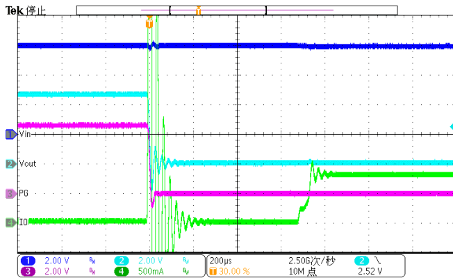
Figure 43. Enter Over Current Protection (Iload=1A)
