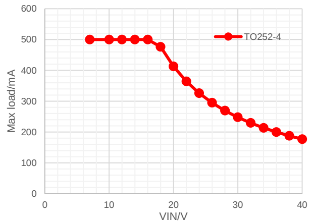
Figure 30. Maximum Output Current vs Input Voltage, VOUT=5V of TO252-4L, T_J \leq TSD\_R (4-layer EVM)
