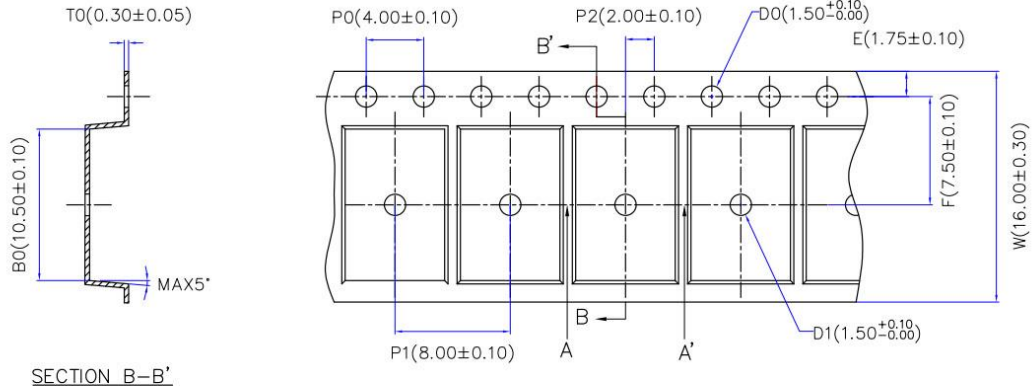
SECTION B-B'
