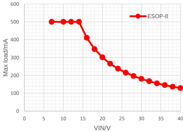
Figure 29. Maximum Output Current vs Input Voltage, VOUT=5V of ESOP-8L, T_J \leq TSD\_R (4-layer EVM)
