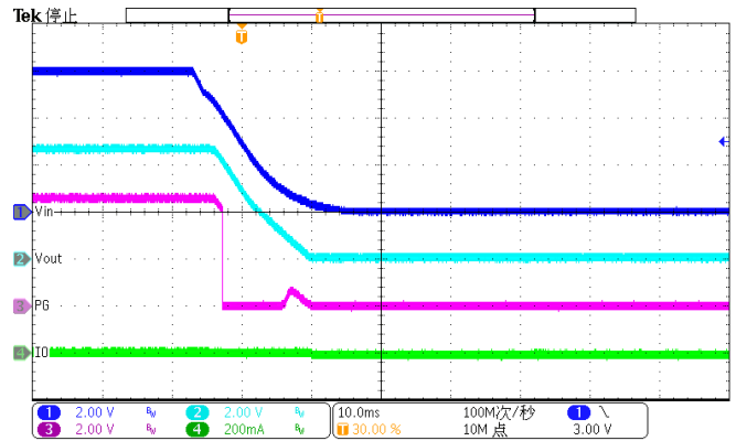
Figure 36. Power down (Iload=10mA)
