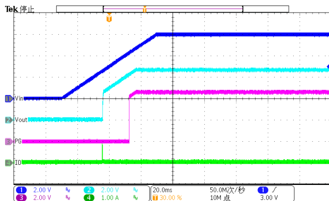
Figure 37. Slow Power up (Iload=10mA)
