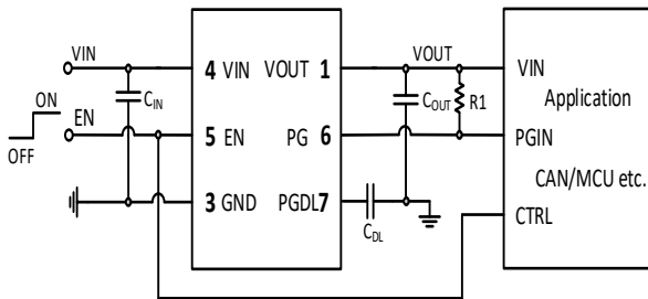
Figure 22. PG Connected to LDO's Output
