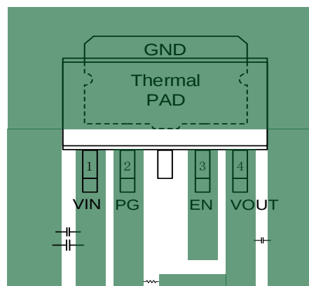
Figure 50. PCB Layout Example
