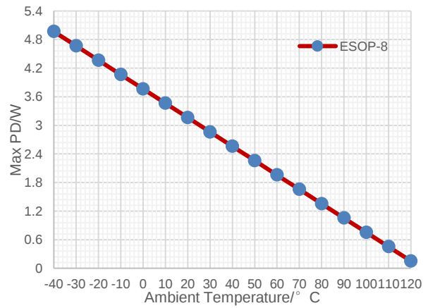
Figure 32. Maximum Allowed Power Dissipation vs Ambient Temperature, ESOP-8L, T_J \leq 125^\circ\text{C} (4-layer EVM)
