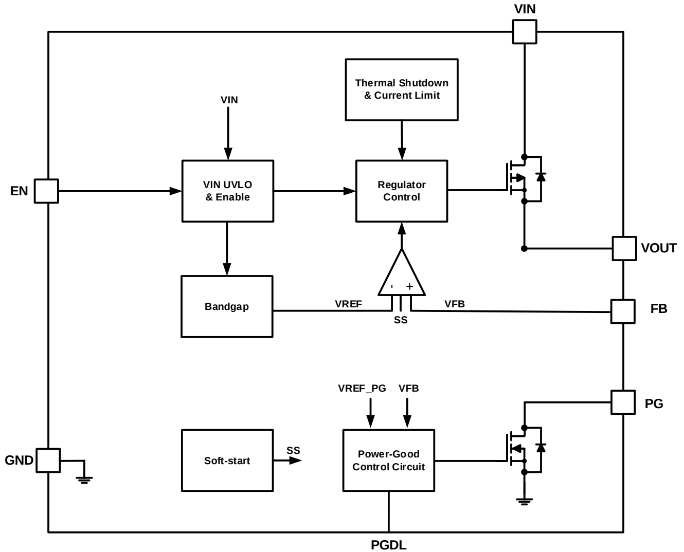
Figure 18. Adjustable Output Version Functional Block Diagram
