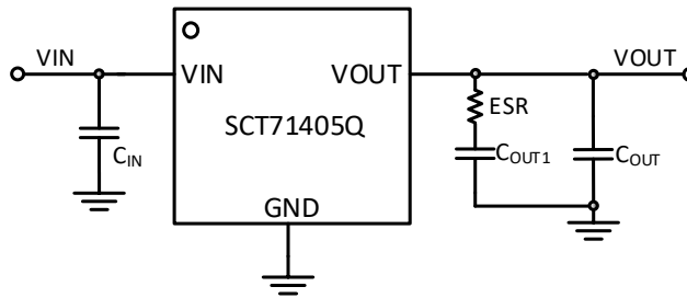
Figure 27. SCT71405Q Typical Application Schematic with Large Output Capacitor
