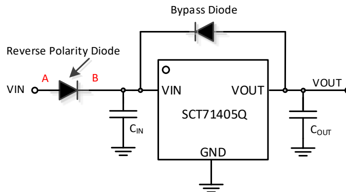
Figure 26. SCT71405Q Typical Application Schematic with Reverse Polarity Diode
