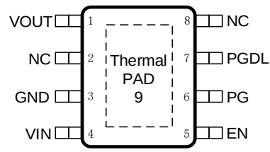
SCT71405FxxBQSTER ESOP-8L Package
