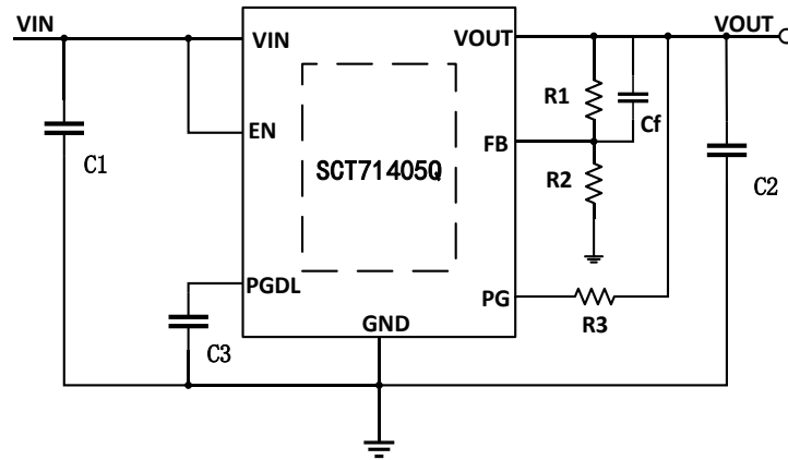
Figure 25. SCT71405Q Typical Application Schematic
