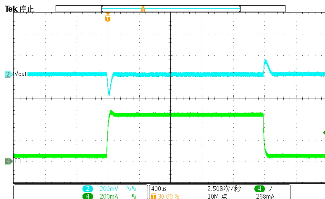
Figure 39. DC-DC Load Transient (50mA-450mA), V_{OUT} = 5V
