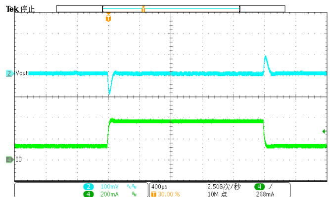
Figure 40. DC-DC Load Transient (130mA-370mA), V_{OUT} = 5V
