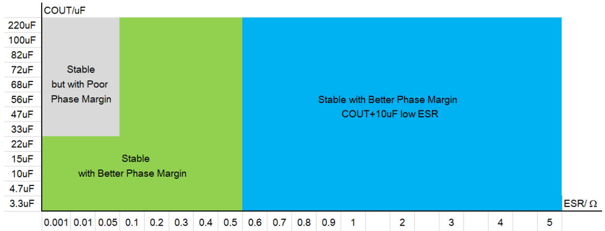
Figure 28. SCT71405Q Stability VS Output Capacitor
