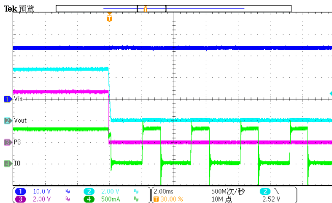
Figure 45. Enter Over Temperature Protection (Vin=24V)
