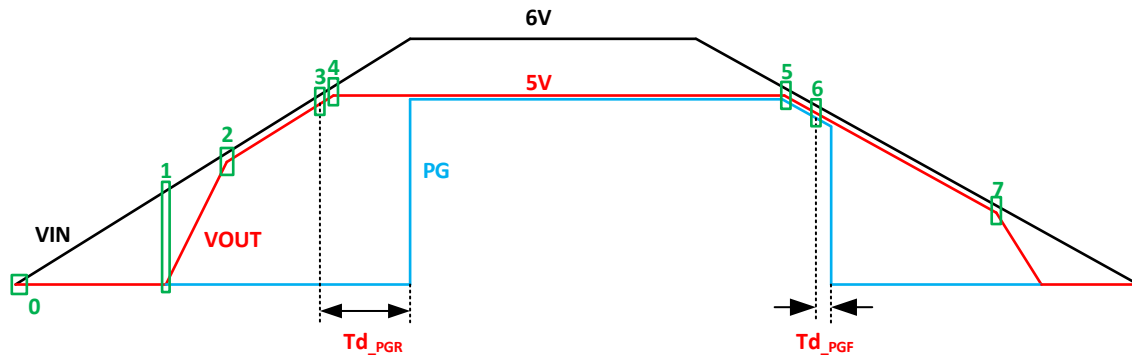
Figure 24. Startup and Shutdown Example —SCT71405Q Series
