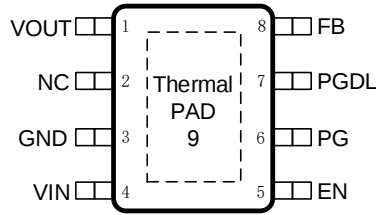
SCT71405A00QSTER ESOP-8L Package
