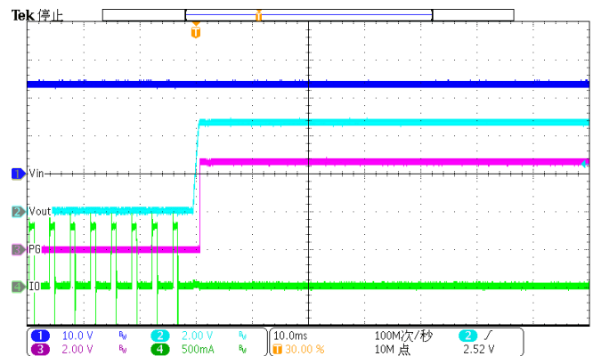
Figure 46. Exit Over Temperature Protection (Vin=24V)
