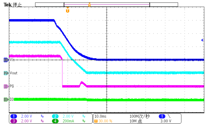
Figure 38. Slow Power down (Iload=10mA)
