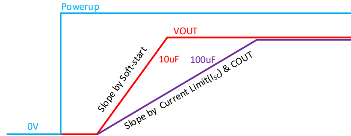
Figure 21. Soft-start Waveform vs Output Capacitor
