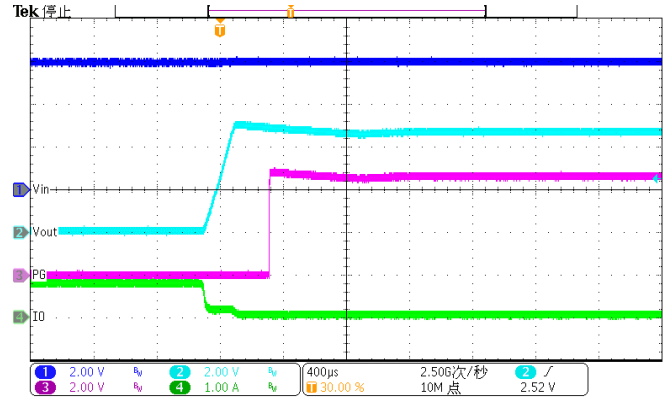
Figure 44. Exit Over Current Protection (Iload=1A)
