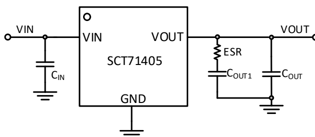
Figure 27. SCT71405 Typical Application Schematic with Large Output Capacitor
