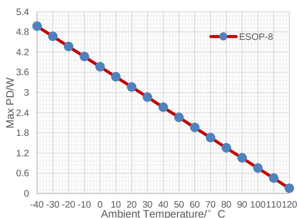
Figure 32. Maximum Allowed Power Dissipation vs Ambient Temperature, ESOP-8L, T_J \leq 125^\circ\text{C} (4-layer EVM)
