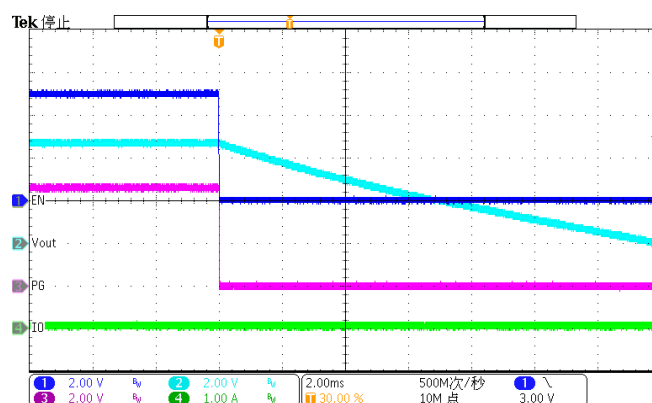
Figure 42. Disable (Iload=10mA)
