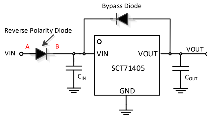
Figure 26. SCT71405 Typical Application Schematic with Reverse Polarity Diode
