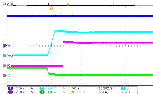
Figure 44. Exit Over Current Protection (Iload=1A)
