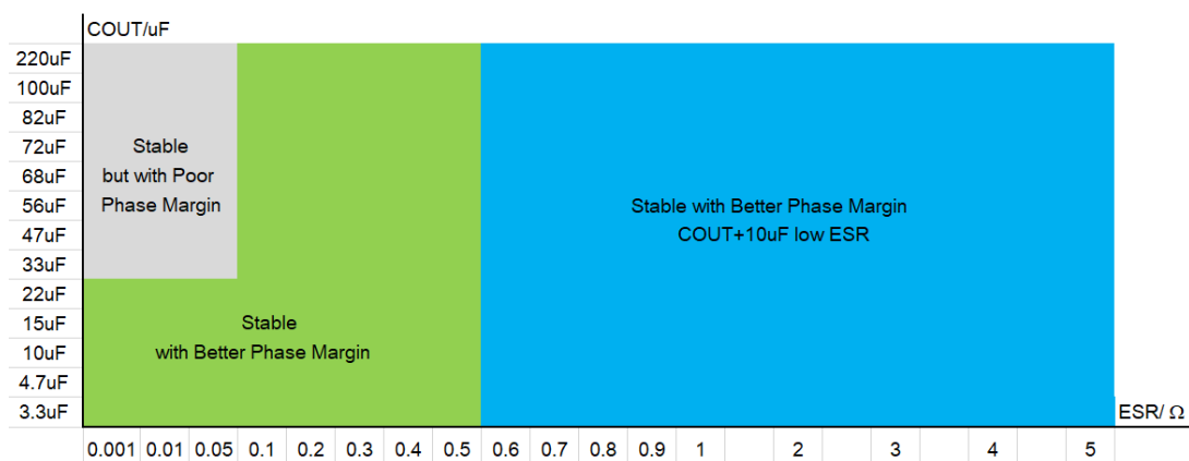
Figure 28. SCT71405 Stability VS Output Capacitor
