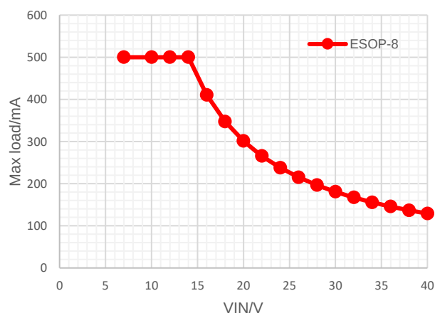
Figure 29. Maximum Output Current vs Input Voltage, VOUT=5V of ESOP-8L, T_J \leq T_{SD\_R} (4-layer EVM)
