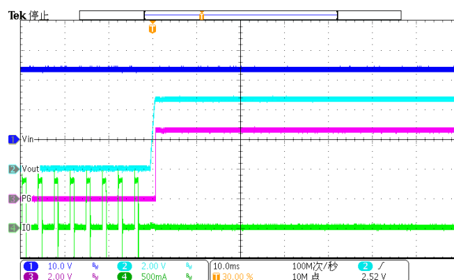
Figure 46. Exit Over Temperature Protection (Vin=24V)
