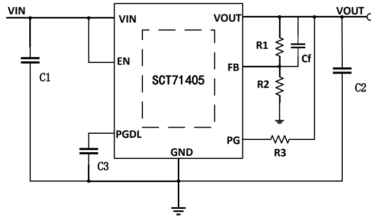
Figure 25. SCT71405 Typical Application Schematic
