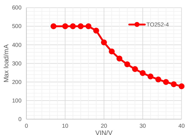
Figure 30. Maximum Output Current vs Input Voltage, VOUT=5V of TO252-4L, T_J \leq T_{SD\_R} (4-layer EVM)
