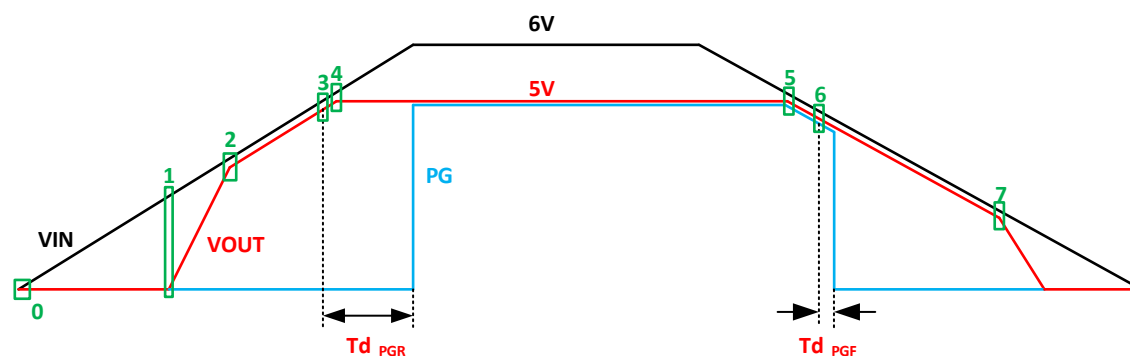
Figure 24. Startup and Shutdown Example —SCT71405 Series
