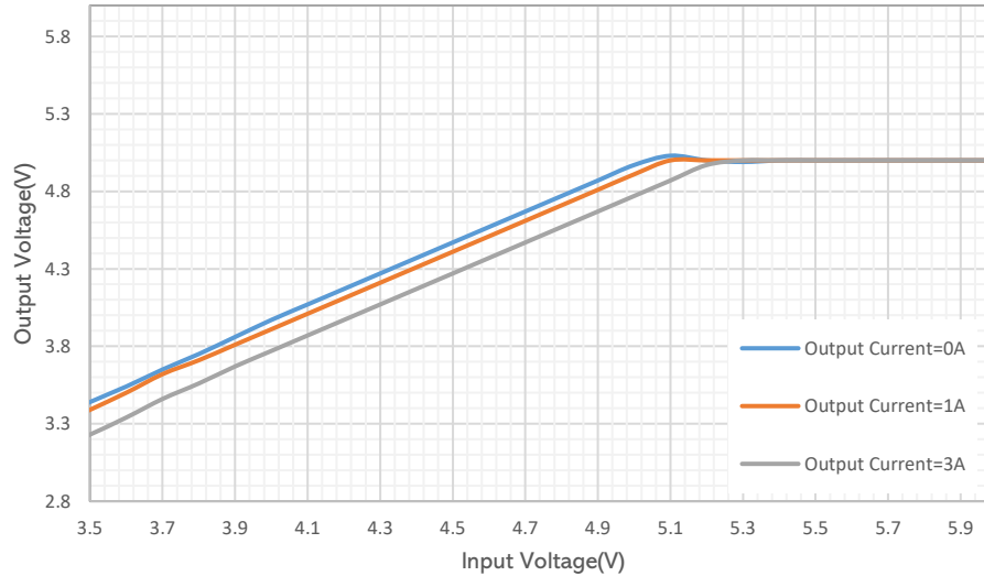
Figure 11. LDO Operation Characteristic (Vout =5V)
