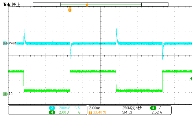
Figure 19. Load Transient (0.4A-3.6A, 1.6A/us)
