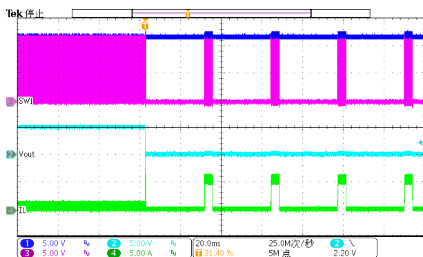
Figure 17. Over Current Protection (0.1A to hard short)
