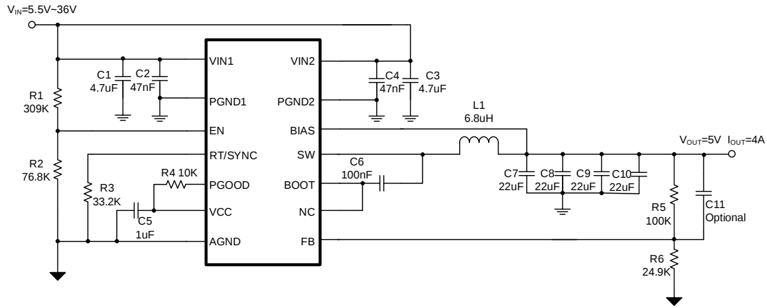
Figure 12. SCT2444Q Design Example, 5V Output with Adjustable UVLO
