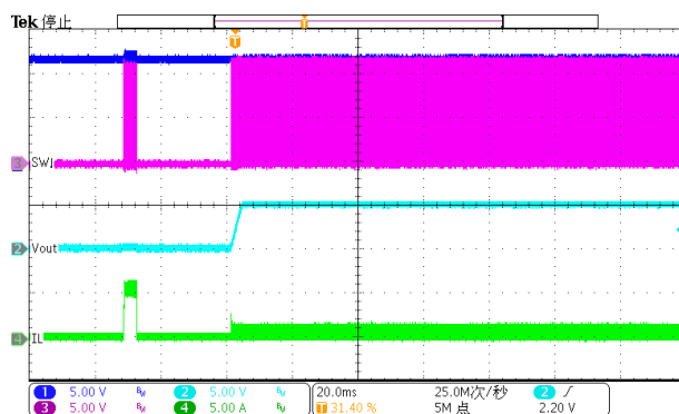
Figure 18. Over Current Release (hard short to 0.1A)
