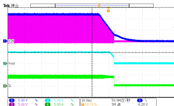
Figure 14. Power down (Iload=4A)
