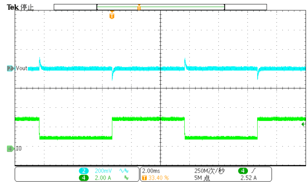
Figure 20. Load Transient (1A-3A, 1.6A/us)
