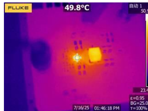
Figure 24. Thermal, 12Vin, 5Vout, 4A
