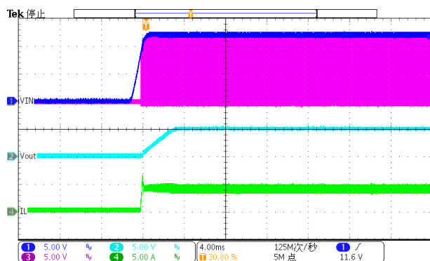
Figure 13. Power up (Iload=4A)
