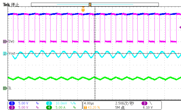
Figure 23. Output Ripple (Iload=4A)
