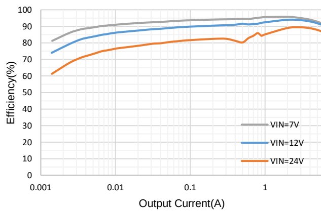
Figure 4. Efficiency, F_{SW}=400KHz , V_{OUT}=3.3V
