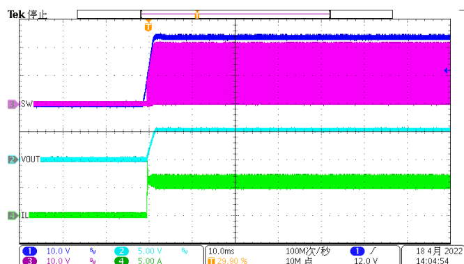
Figure 13. Power up(Iload=6A)
