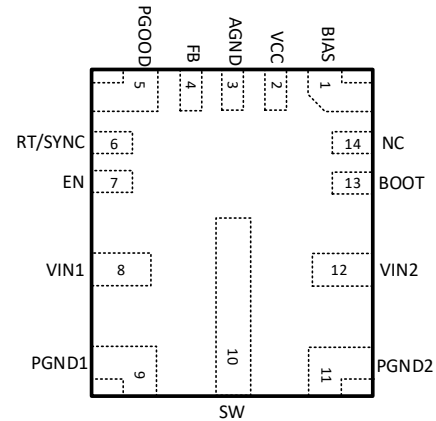
Figure 1. 14-Lead FCQFN 3.5mmx4mm
