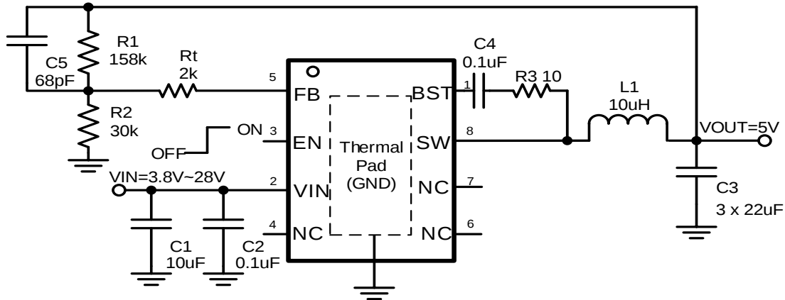
*For input voltage higher than 18V, R3=10 is highly recommend. Figure 11. 24V Input, 5V/5A Output
