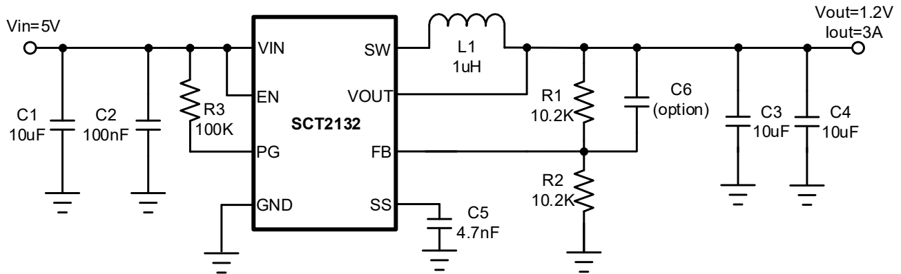
Figure 8. SCT2132 Design Example, 1.2V Output
