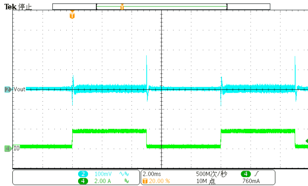
Figure 18. Load Transient (0.2A-1.8A, 1.6A/us)
