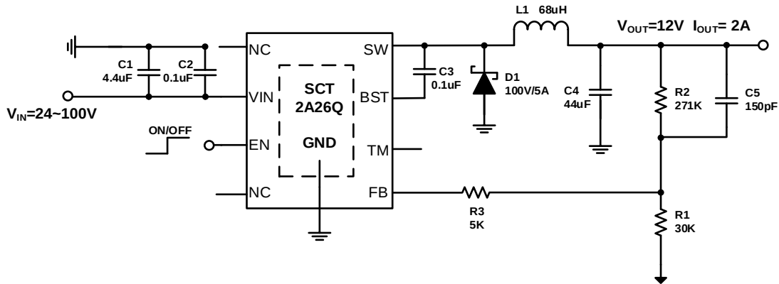
Figure 10. SCT2A26Q Design Example, 12V Output
