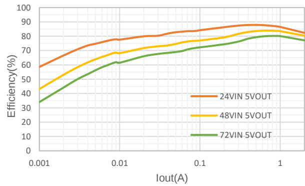
Figure 3. Efficiency vs Load Current, Vout=5V
