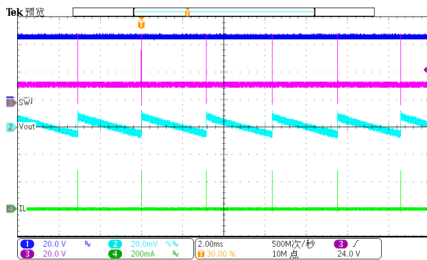
Figure 20. Output Ripple ( I_{load}=0A )
