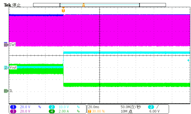
Figure 17. Over Current Release
