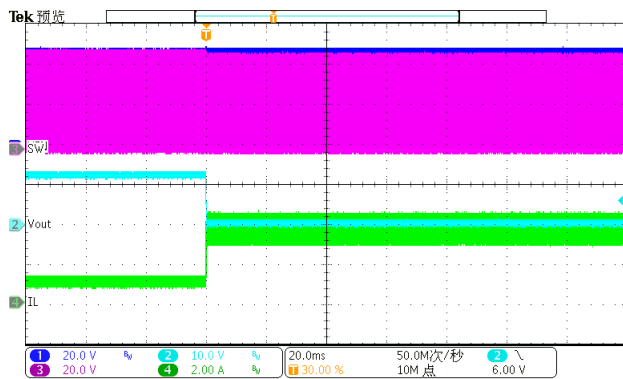
Figure 16. Over Current Protection
