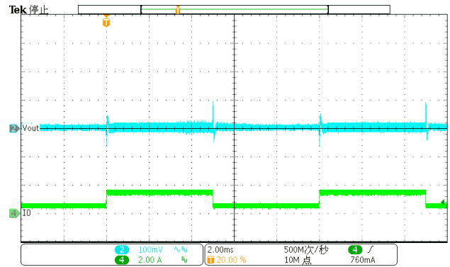
Figure 19. Load Transient (0.75A-1.25A, 1.6A/us)
