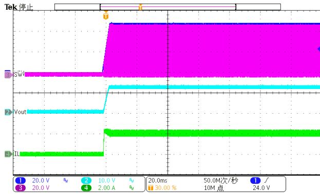
Figure 12. Power up (Iload=2A)
