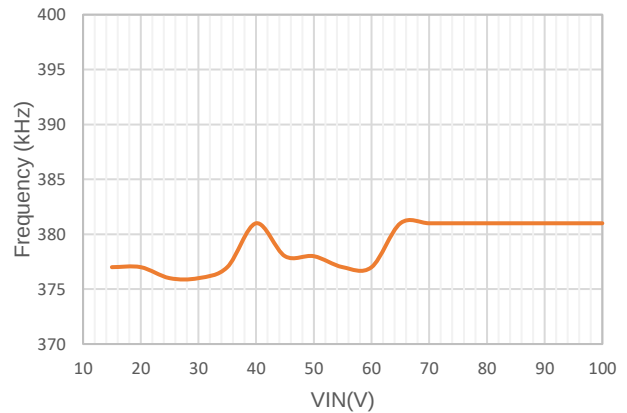
Figure 7. Switching Frequency vs Vin, Vout=12V
