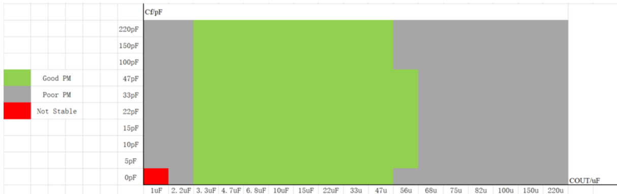
Figure 26. SCT71601Q Feed Forward Capacitors recommend( R_2=10k\Omega , V_{OUT}=1.8V )
