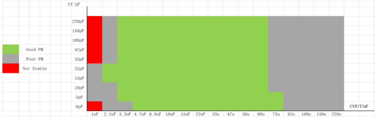
Figure 25. SCT71601Q Feed Forward Capacitors recommend( R_2=100k\Omega , V_{OUT}=1.8V )
