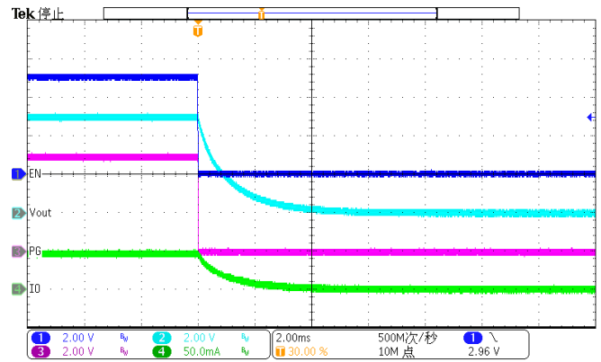
Figure 39. Disable (Iload=50mA)
