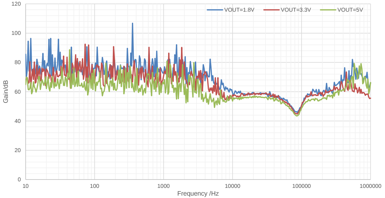
Figure 13. PSRR vs Frequency VIN=12V, Cf=10pF, COUT=10uF, IOUT=10mA
