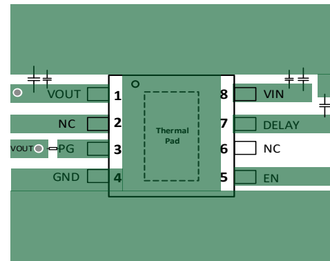
Figure 45. PCB Layout Example
