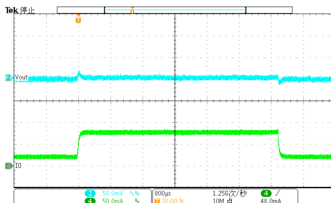
Figure 37. DC-DC Load Transient (25mA-75mA), V_{OUT} = 5V
