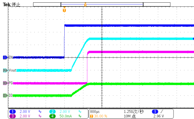
Figure 38. Enable (Iload=50mA)
