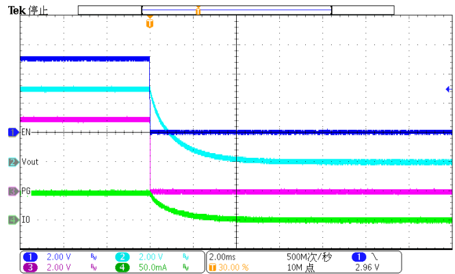
Figure 39. Disable (Iload=50mA)
