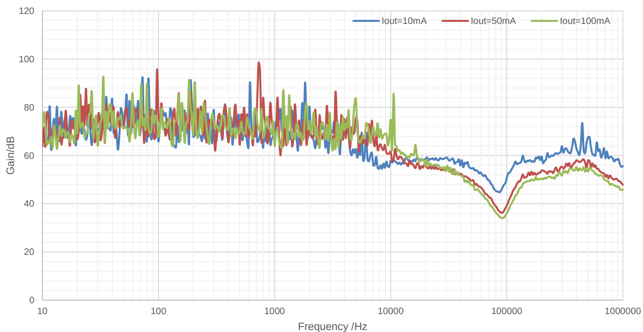
Figure 14. PSRR vs Frequency VIN=12V, VOUT=3.3V, Cf=10pF, COUT=10uF
