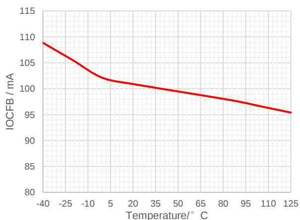
Figure 10. Output Current Limit vs Ambient Temperature at VIN≥55V
