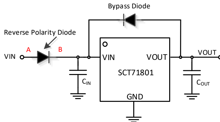
Figure 23. SCT71801A00 Typical Application Schematic with Reverse Polarity Diode
