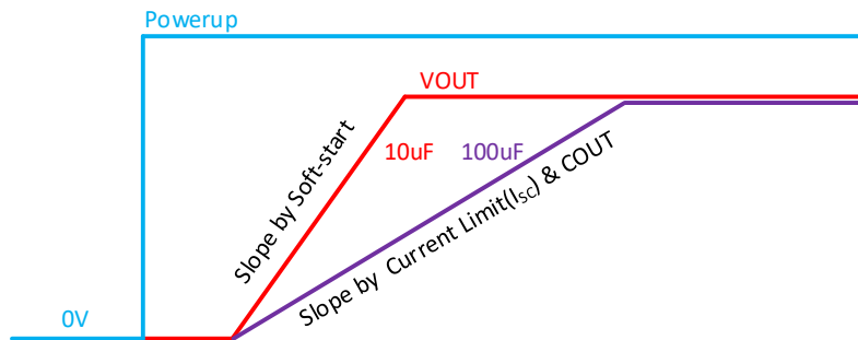
Figure 18. Soft-start Waveform vs Output Capacitor
