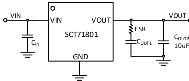
Figure 24. SCT71801A00 Typical Application Schematic with Large Output Capacitor
