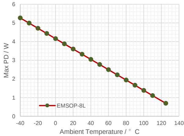
Figure 30. Maximum Allowed Power Dissipation vs Ambient Temperature, EMSOP-8L, T_J \leq 150^\circ\text{C}
