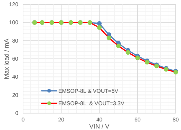
Figure 31. Maximum Output Current vs Input Voltage, EMSOP-8L, T_J \leq 150^\circ\text{C}
