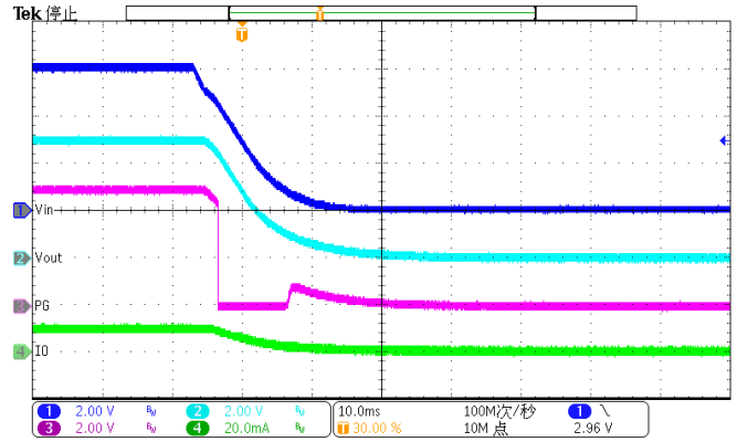
Figure 33. Power down ( PG pin pulled up to V_{OUT} )
