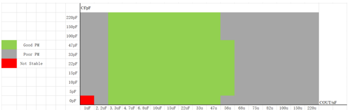
Figure 26. SCT71801A00 Feed Forward Capacitors recommend( R_2=10k\Omega , V_{OUT}=1.8V )
