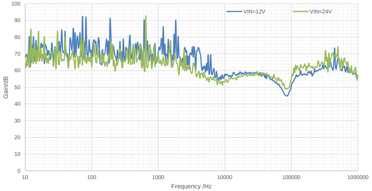
Figure 11. PSRR vs Frequency V_{OUT}=3.3V, C_f=10pF, C_{OUT}=10\mu F, I_{OUT}=10mA
