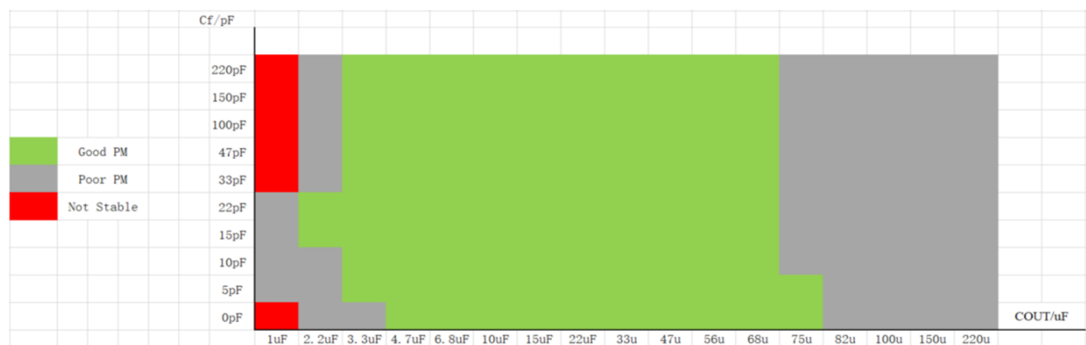
Figure 25. SCT71801A00 Feed Forward Capacitors recommend( R_2=100k\Omega , V_{OUT}=1.8V )
