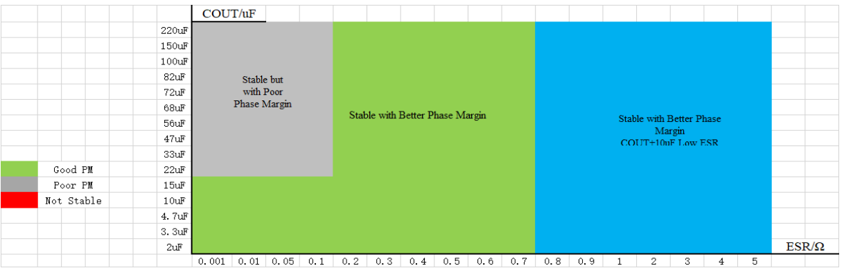
Figure 27. SCT71801A00 Stability VS Output Capacitor
