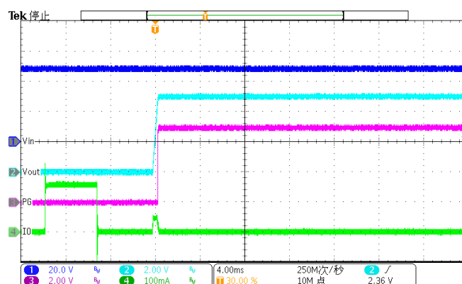
Figure 43. Exit Over Temperature Protection(Vin=48V)
