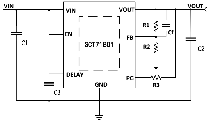
Figure 22. SCT71801A00 Typical Application Schematic
