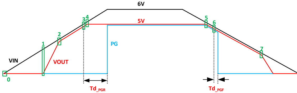
Figure 21. Startup and Shutdown Example —SCT71801A00 Series
