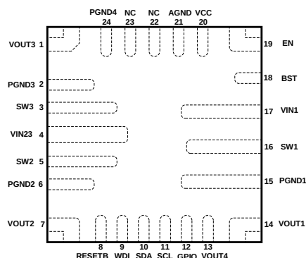
Top View: 24-Lead FCQFN 4mmx4mm
