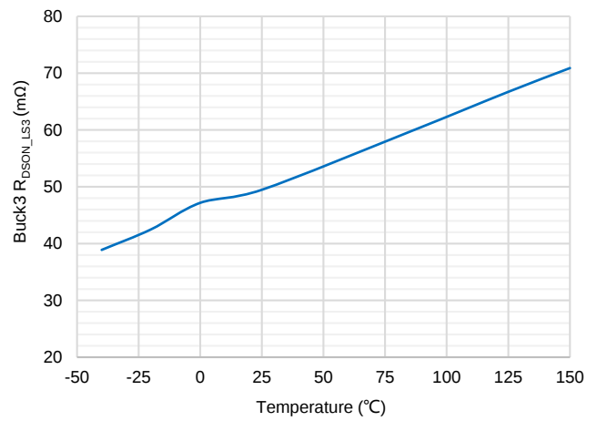
Buck3 R DSON_LS3 vs. Temperature
