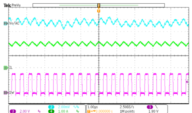
Figure 13. Buck2 Steady State ( I_{o2} = 2A )
