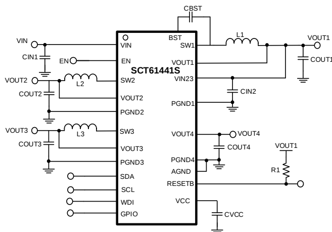
SCT61441S PMIC Typical Application Circuit
