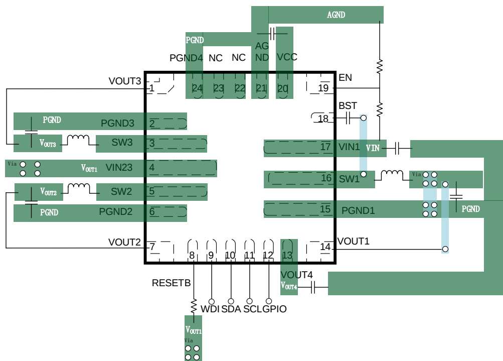
Figure 15. PCB Layout Example
