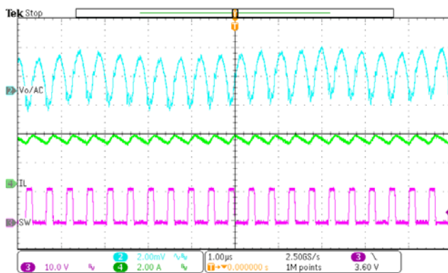
Figure 12. Buck1 Steady State ( I_{o1} = 3A )
