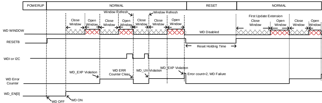
Figure 3a. Simple Watchdog Error Timing
