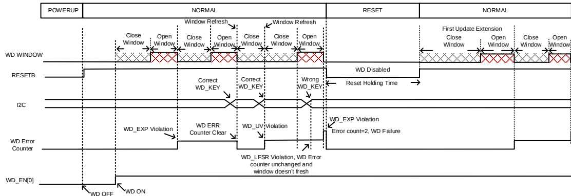
Figure 3b. QA Watchdog Error Timing
