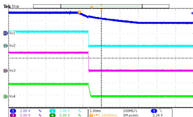
Figure 13. Power Off ( I_{O2}=I_{O3}=2A , I_{O4}=0.5A , I_{O5}=0.8A )
