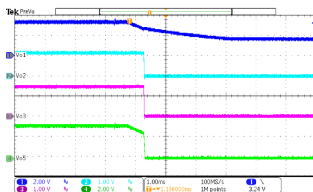
Figure 14. Power Off ( I_{O2}=I_{O3}=2A , I_{O4}=0.5A , I_{O5}=0.8A )
