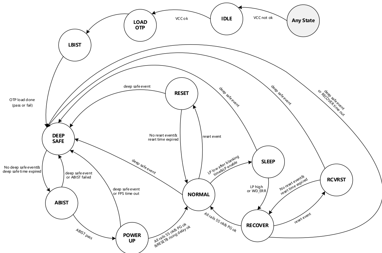
Figure 2. Operating State Transitions
