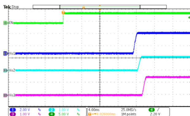
Figure 15. EN On ( I_{O2}=I_{O3}=2A , I_{O4}=0.5A , I_{O5}=0.8A )
