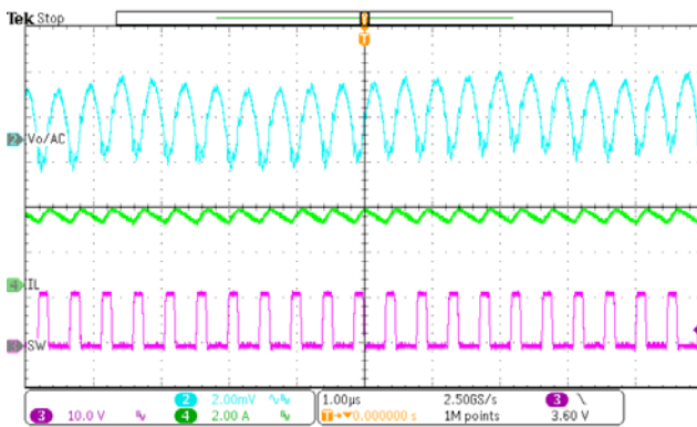
Figure19. Buck1 Steady State ( I_{o1} = 3A )
