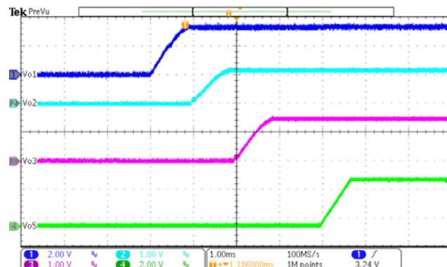
Figure 12. Power On ( I_{O2}=I_{O3}=2A , I_{O4}=0.5A , I_{O5}=0.8A )
