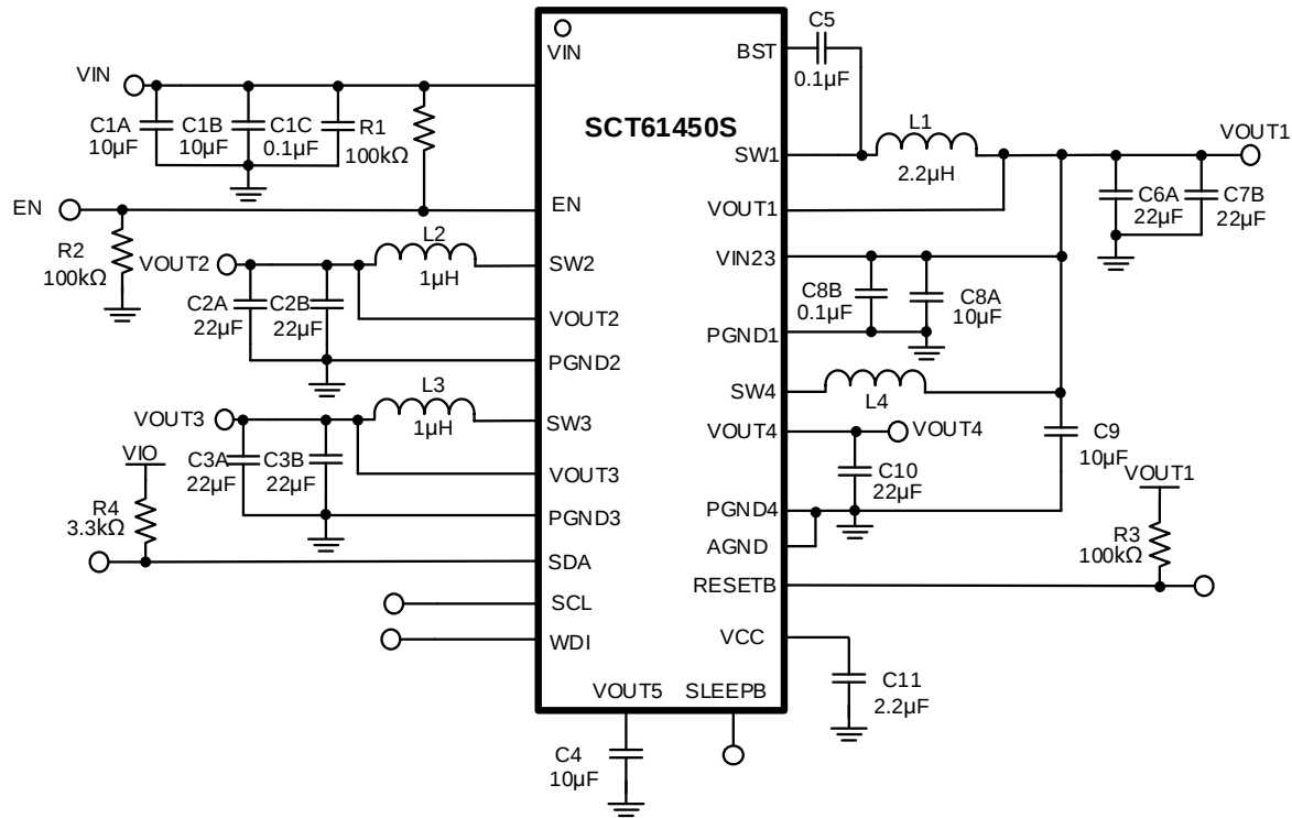
Figure 9. Application Schematic, 3.5V to 36V, PMIC Regulator at 2.2MHz
