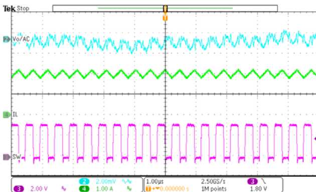
Figure 21. Buck3 Steady State ( I_{o3} = 2A )
