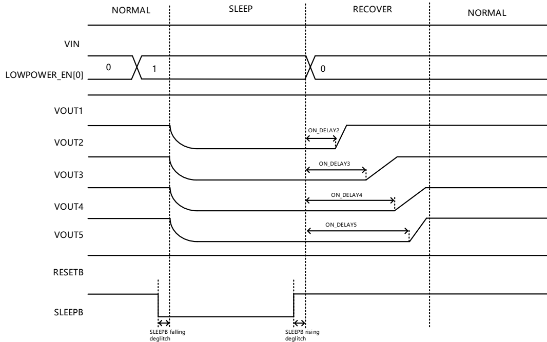
Figure 8. Sleep Mode Entry and Exit Diagram
