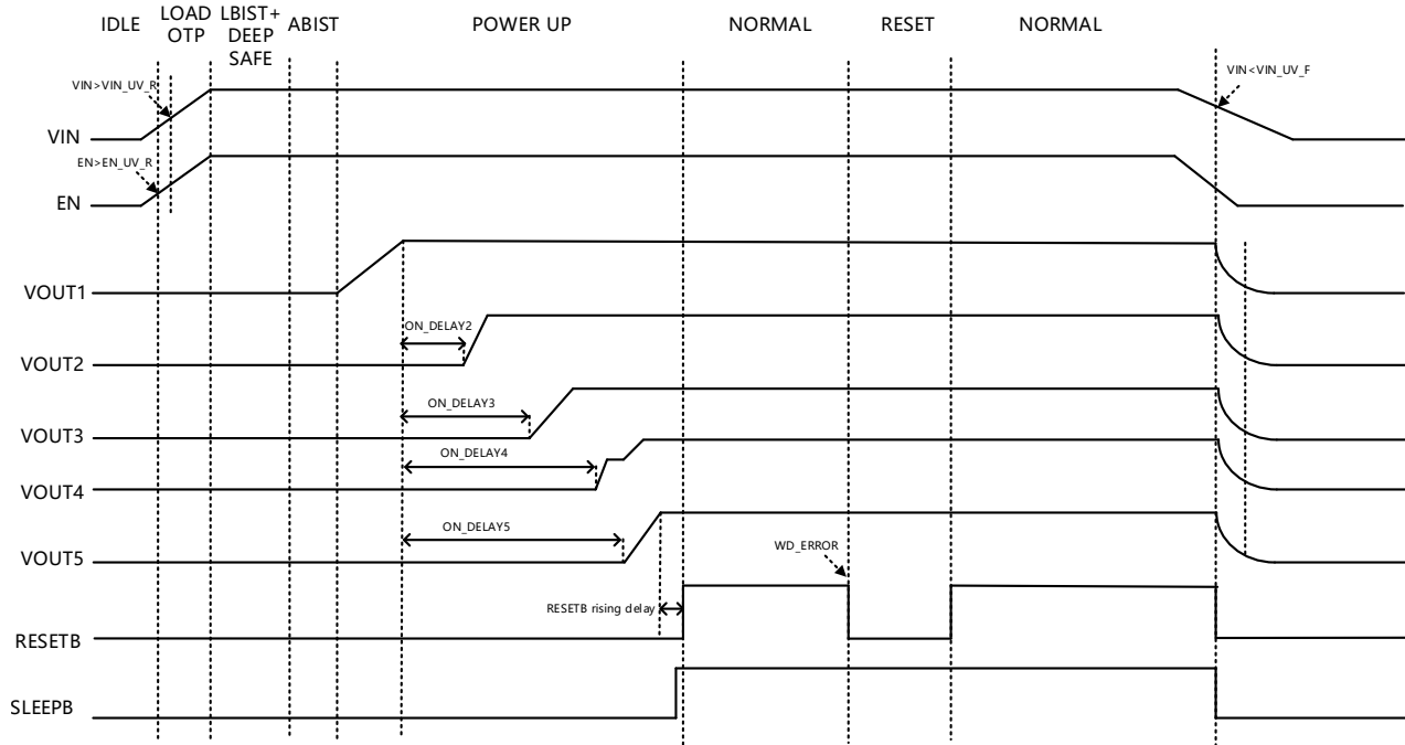
Figure 7. Power on Sequence
