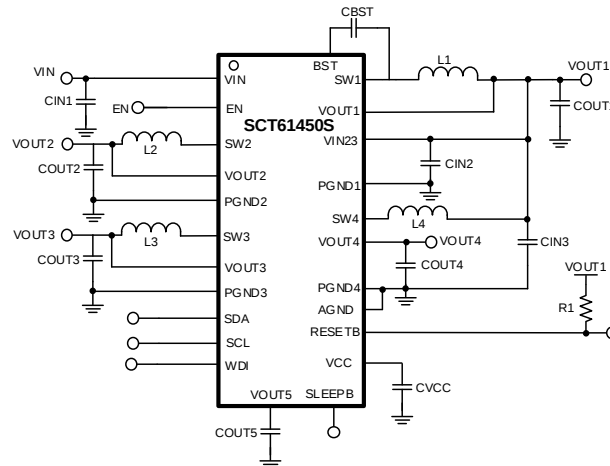
SCT61450S Radar PMIC Typical Application Circuit
