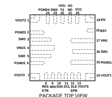
Top View: 24-Lead FCQFN 4mmx4mm
