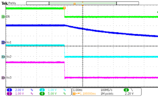
Figure 17. EN Off ( I_{o2}=I_{o3}=2A , I_{o4}=0.5A , I_{o5}=0.8A )
