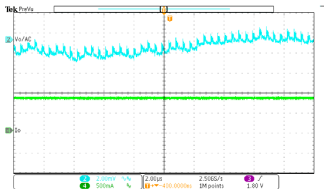
Figure 23. Loadswitch Steady State ( I_{o5} = 800mA )
