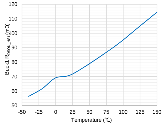
Buck1 R_{DSON\_HS1} vs. Temperature
