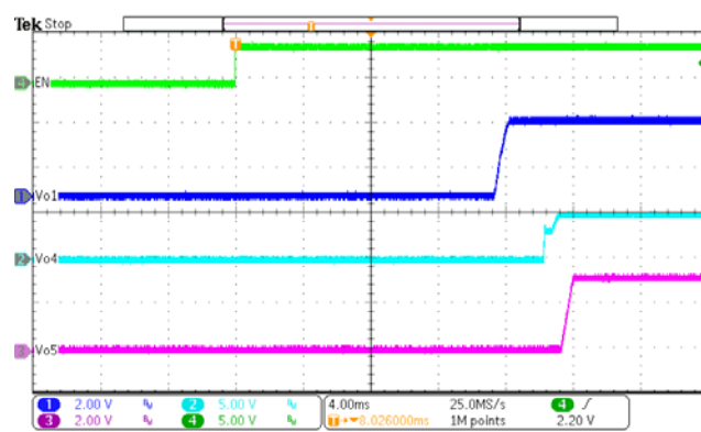
Figure 16. EN On ( I_{O2}=I_{O3}=2A , I_{O4}=0.5A , I_{O5}=0.8A )
