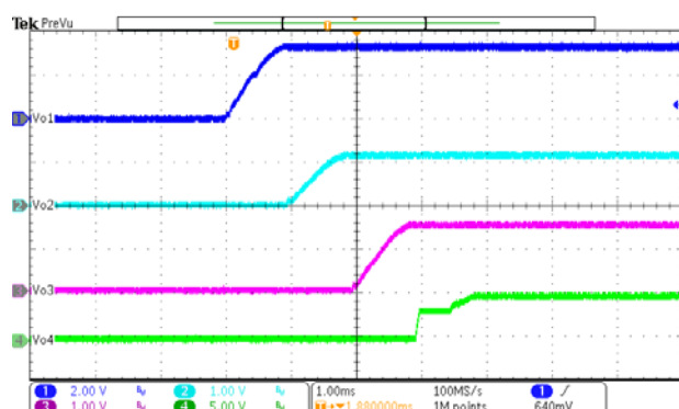
Figure 11. Power On ( I_{O2}=I_{O3}=2A , I_{O4}=0.5A , I_{O5}=0.8A )
