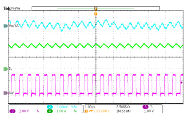
Figure 15. Buck2 Steady State ( I_{O2} = 2A )
