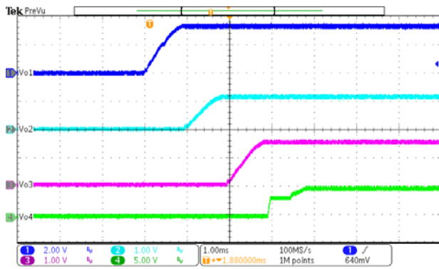
Figure 10. Power On ( I_{O2}=I_{O3}=2A , I_{O4}=0.5A )
