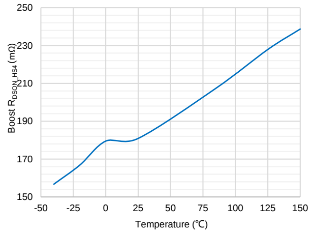
Boost R_{DS(on)_HS4} vs. Temperature
