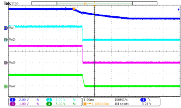
Figure 11. Power Off ( I_{O2}=I_{O3}=2A , I_{O4}=0.5A )
