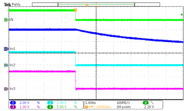
Figure 13. EN Off ( I_{O2}=I_{O3}=2A , I_{O4}=0.5A )
