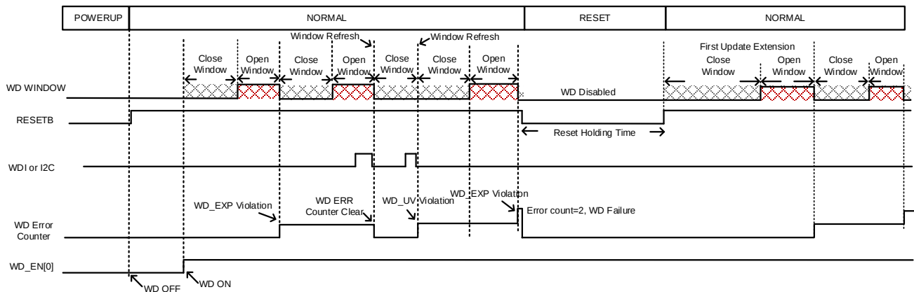
Simple Mode With WD OFF by Default
