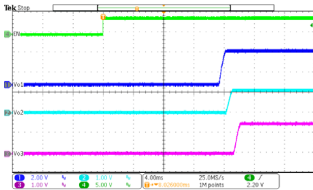
Figure 12. EN On ( I_{O2}=I_{O3}=2A , I_{O4}=0.5A )
