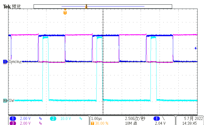
Figure 40. SYNCIN and SYNCOUT
