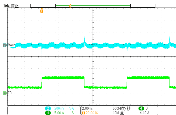
Figure 36. Load Transient (2A-6A, 1.6A/us)
