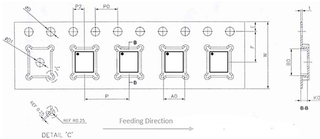
TAPE DIMENSIONS
