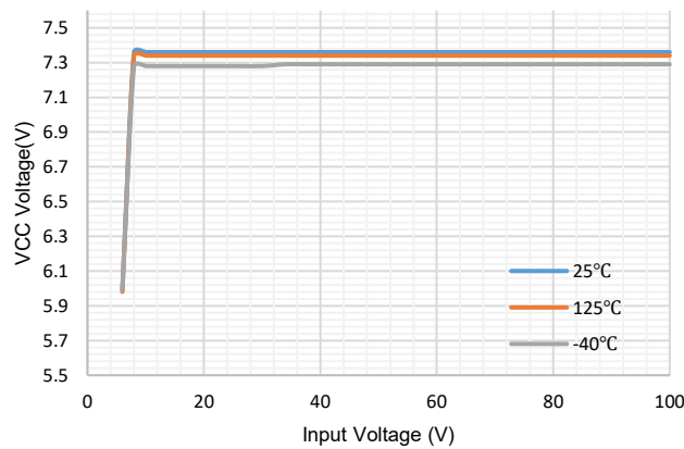
Figure 17. VCC Voltage vs Input Voltage
