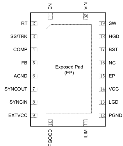
Top View: DFN3.5X4.5-20L
