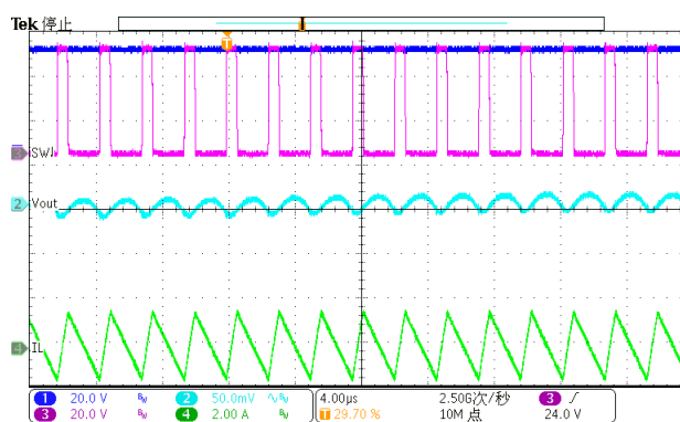
Figure 38. Output Ripple, FCCM (Iload=100mA)
