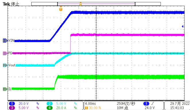
Figure 42. Power up(Iload=20A)
