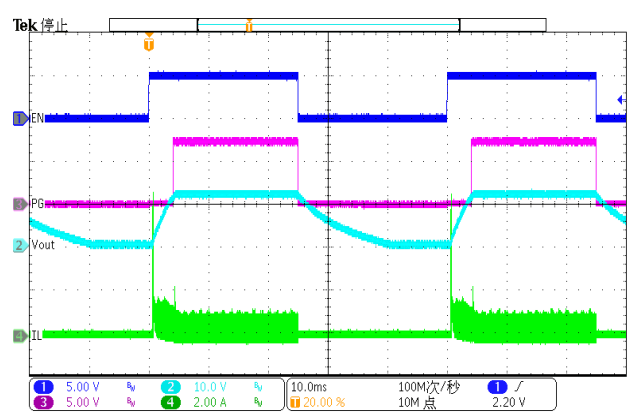
Figure 32. Enable (Iload=0.1A)
