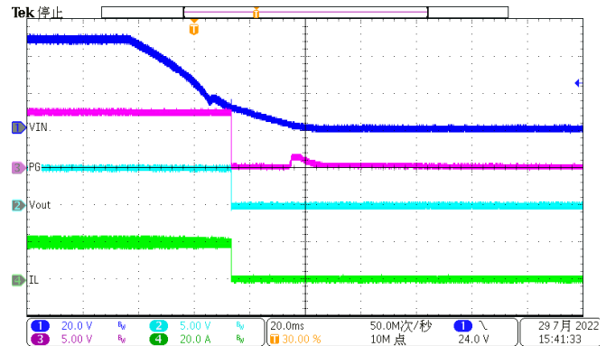
Figure 43. Power down(Iload=20A)
