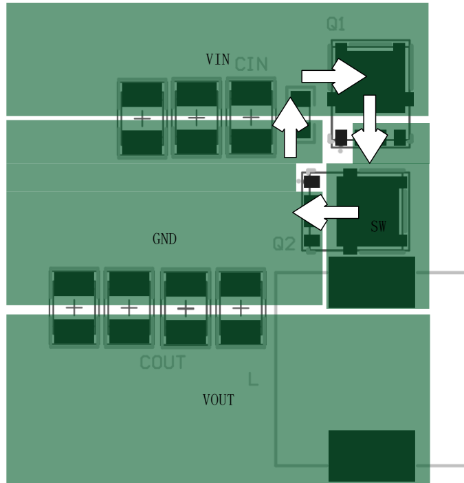
Figure 54. Power stage PCB Layout
