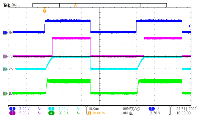
Figure 44. Enable (Iload=20A)
