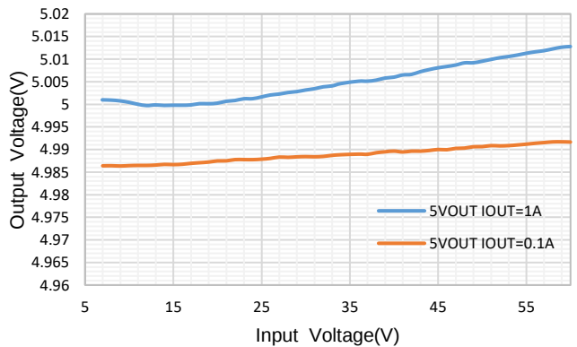
Figure 6. Line Regulation
