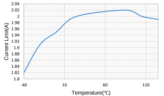
Figure 7. HS Current Limit VS Temperature
