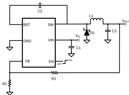
4.5V-60V, Asynchronous Buck Converter
