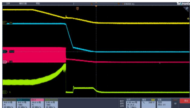
Figure 23. Power down ( I_{LOAD}=2A )
