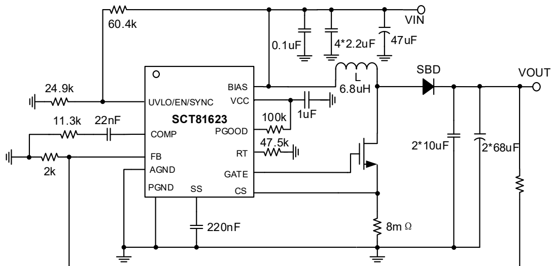
Figure 21. Application Schematic, 6V to 18V, 2A Boost Regulator at 456kHz
