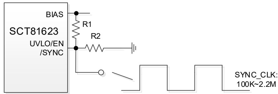
Figure 20. Frequency Sync
