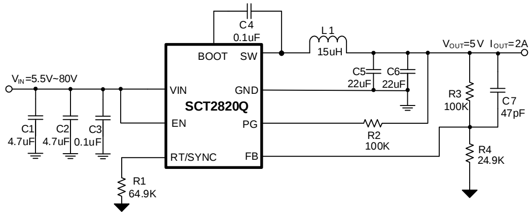
Figure 11. SCT2820Q Design Example, 5V Output
