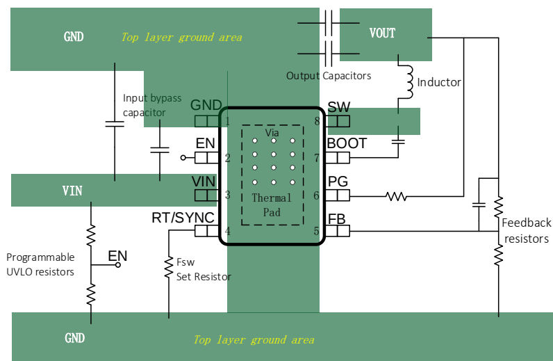
Figure 24. PCB Layout Example
