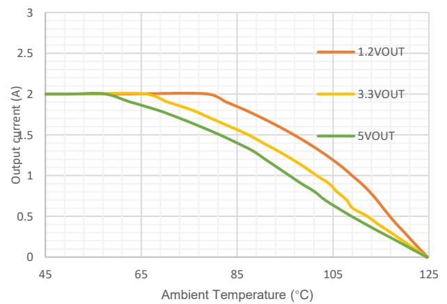
Figure 6. Thermal Derating, VIN=12V ( \theta_{JA}=60^{\circ}\text{C/W} )
