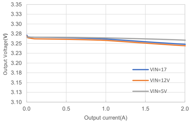
Figure 3. Load Regulation
