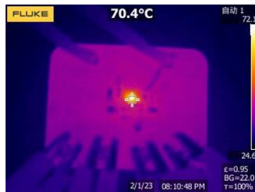
Figure 20. Thermal, 3.3Vout/2A
