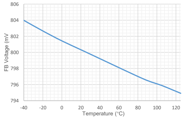
Figure 4. FB Voltage Vs. Temperature
