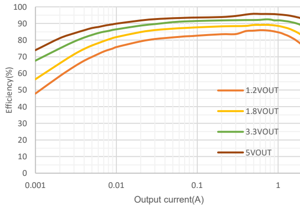
Figure 1. Efficiency vs Load Current(VIN=7.2V)
