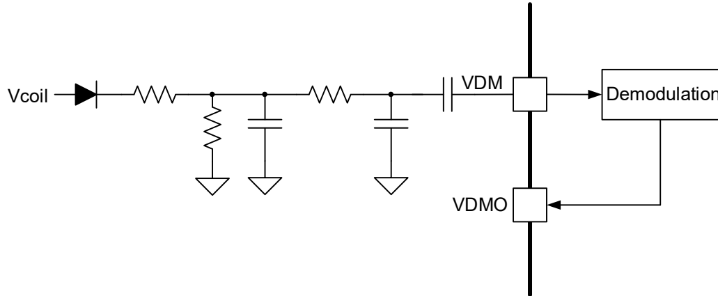
Figure 10. Envelope Detector
