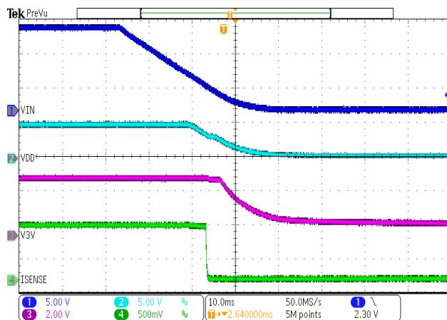
Figure 13. Power Down
