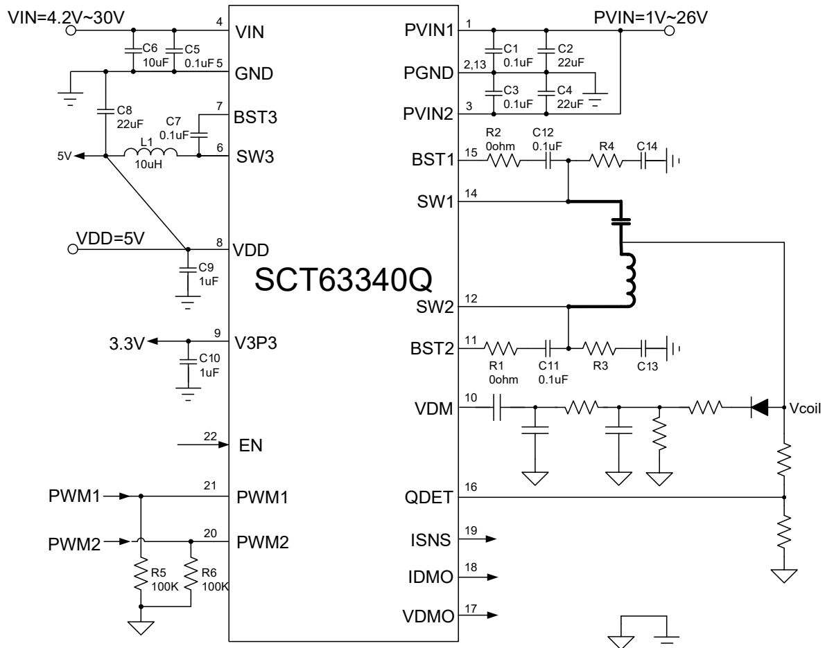
Figure 11. Separate Input to VIN and PVIN
