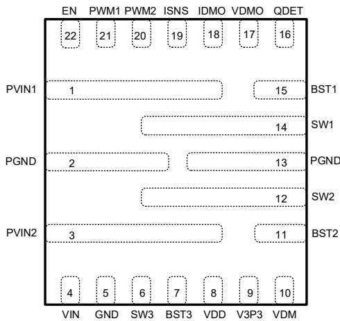
Figure 1. Top view 22-Lead QFN 4mm*4mm
