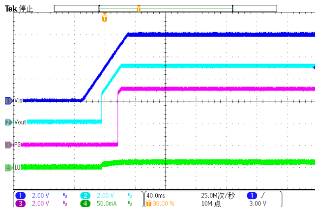
Figure 42 Slow Power up (Iload=10mA)
