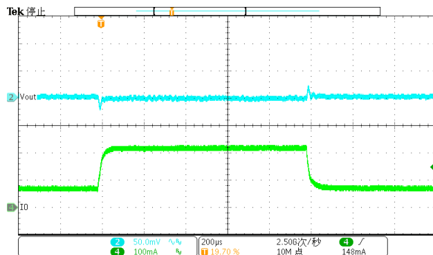
Figure 47. DC-DC Load Transient (75mA-225mA), V_{OUT}=3.3V
