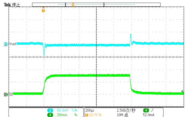
Figure 53. DC-DC Load Transient (1mA-300mA) ,VOUT=3.3V
