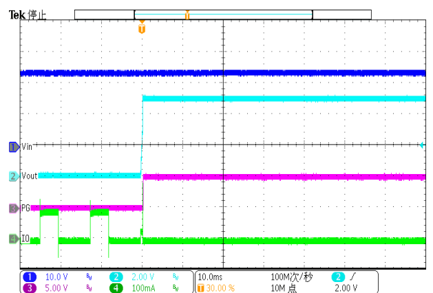
Figure 57. Exit Over Temperature Protection
