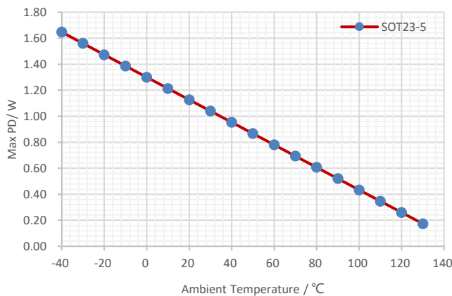
Figure 34. Maximum Allowed Power Dissipation vs Ambient Temperature, SOT23-5L, T_J \leq 150^\circ C
