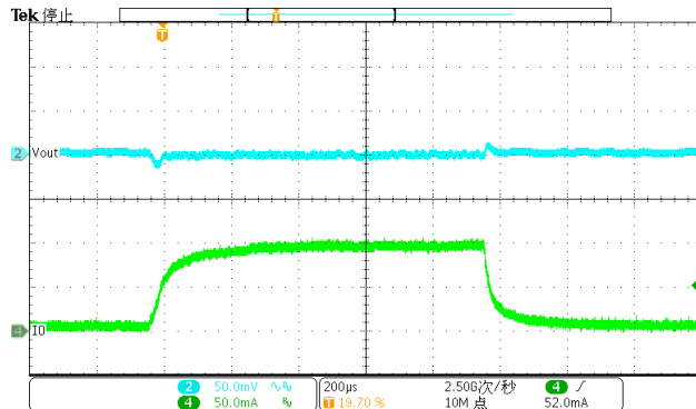
Figure 51. DC-DC Load Transient (1mA-100mA), V_{OUT}=3.3V
