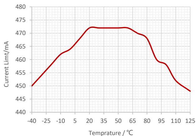
Figure 11. Output Current Limit vs Ambient Temperature
