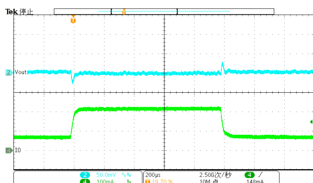
Figure 46. DC-DC Load Transient (75mA-225mA), V_{OUT}=5V
