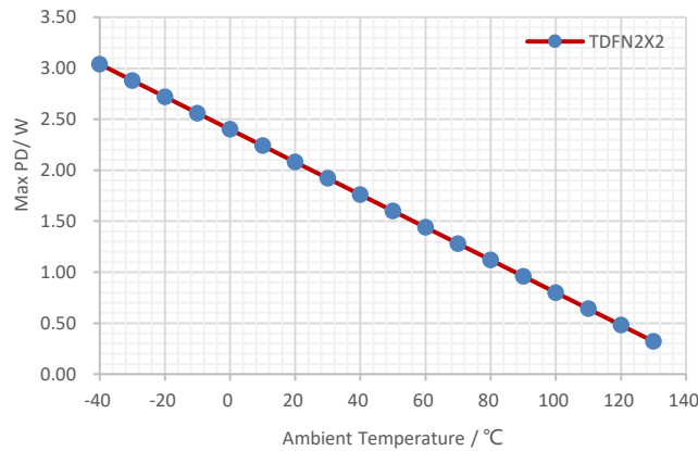
Figure 32. Maximum Allowed Power Dissipation vs Ambient Temperature, DFN2X2, T_J \leq 150^\circ C
