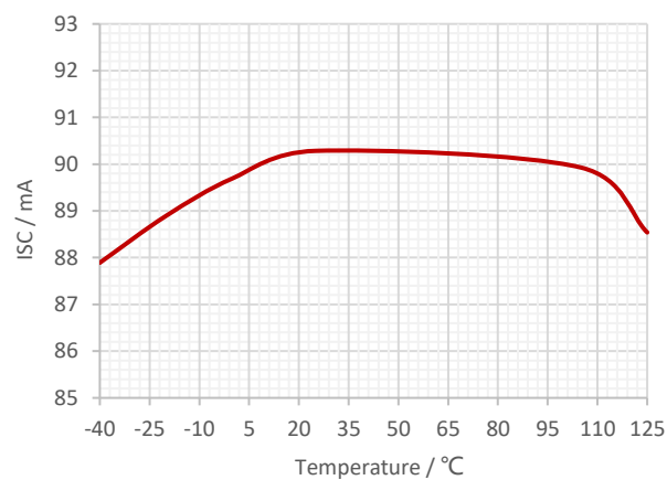
Figure 12. Short Current Limit vs Ambient Temperature
