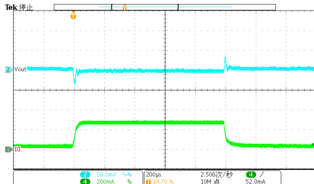
Figure 49. DC-DC Load Transient (30mA-270mA), V_{OUT}=3.3V
