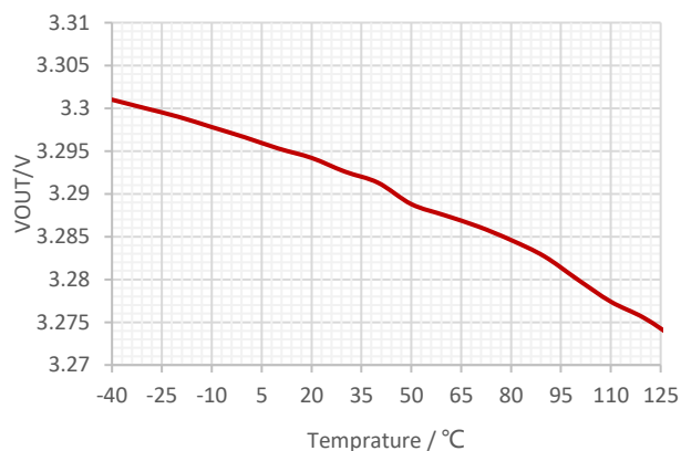
Figure 8. Output Voltage vs Ambient Temperature at VOUT=3.3V
