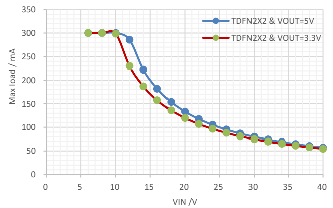
Figure 33. Maximum Output Current vs Input Voltage, DFN2X2, T_J \leq 150^\circ C
