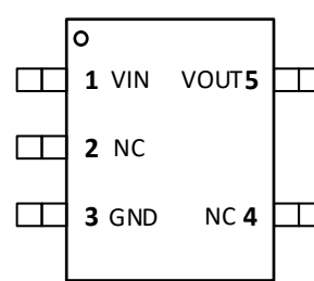
SCT71403FxxTWDR SOT23-5L Package
