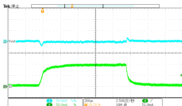
Figure 50. DC-DC Load Transient (1mA-100mA), V_{OUT}=5V
