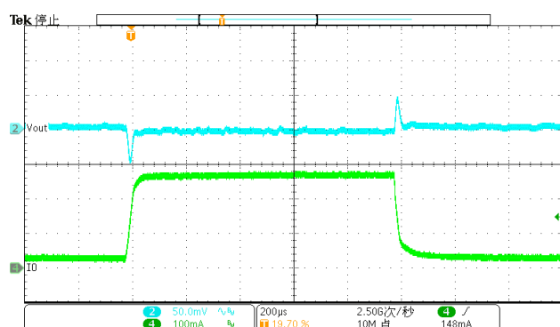
Figure 48. DC-DC Load Transient (30mA-270mA), V_{OUT}=5V
