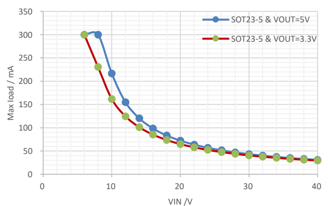
Figure 35. Maximum Output Current vs Input Voltage, SOT23-5L, T_J \leq 150^\circ C
