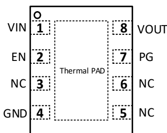
SCT71403FxxDTBR DFN3X3-8L Package
