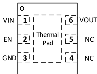
SCT71403FxxDVAR DFN2X2-6L Package
