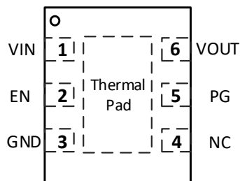
SCT71403FxxADVAR DFN2X2-6L Package
