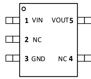
SCT71403FxxQTWDR SOT23-5L Package
