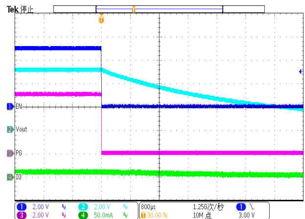
Figure 47. Disable (Iload=10mA)
