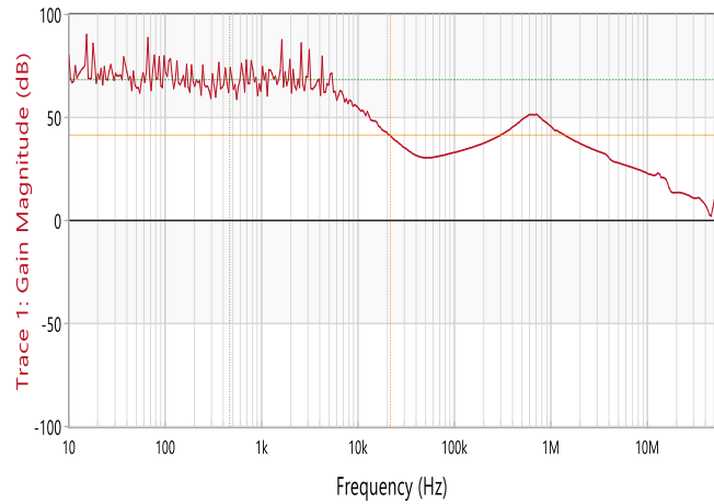
Figure 16. PSRR vs Frequency at Iout=100mA, C OUT =10uF
