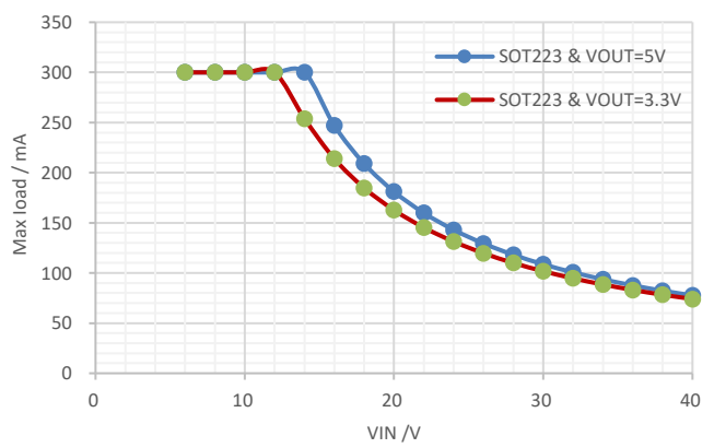
Figure 41. Maximum Output Current vs Input Voltage, SOT223-4L, T_J \leq 150^\circ\text{C}
