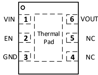
SCT71403FxxQDVAR DFN2X2-6L Package
