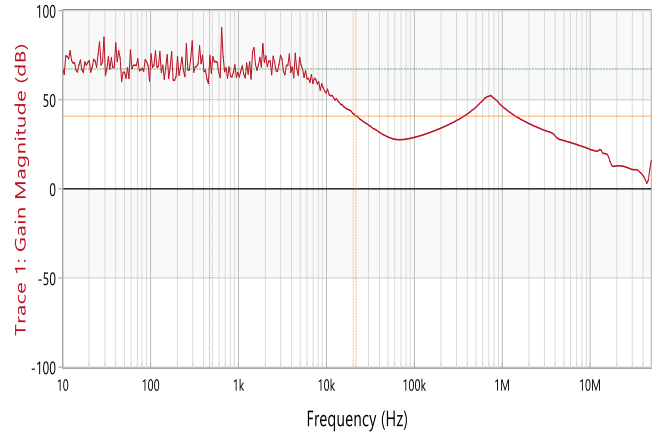
Figure 14. PSRR vs Frequency at Iout=100mA, C OUT =4.7uF
