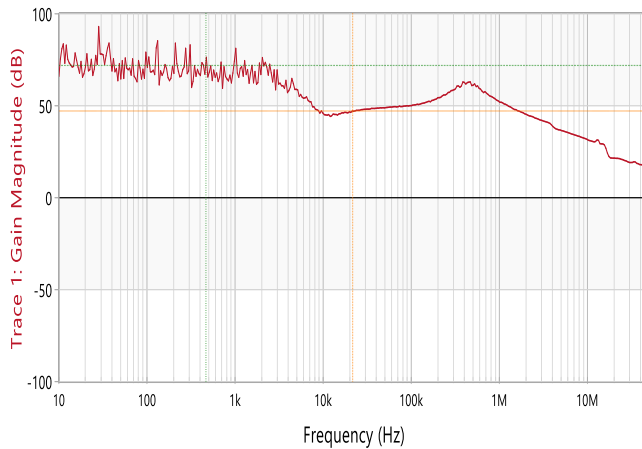
Figure 17. PSRR vs Frequency at Iout=10mA, C OUT =22uF
