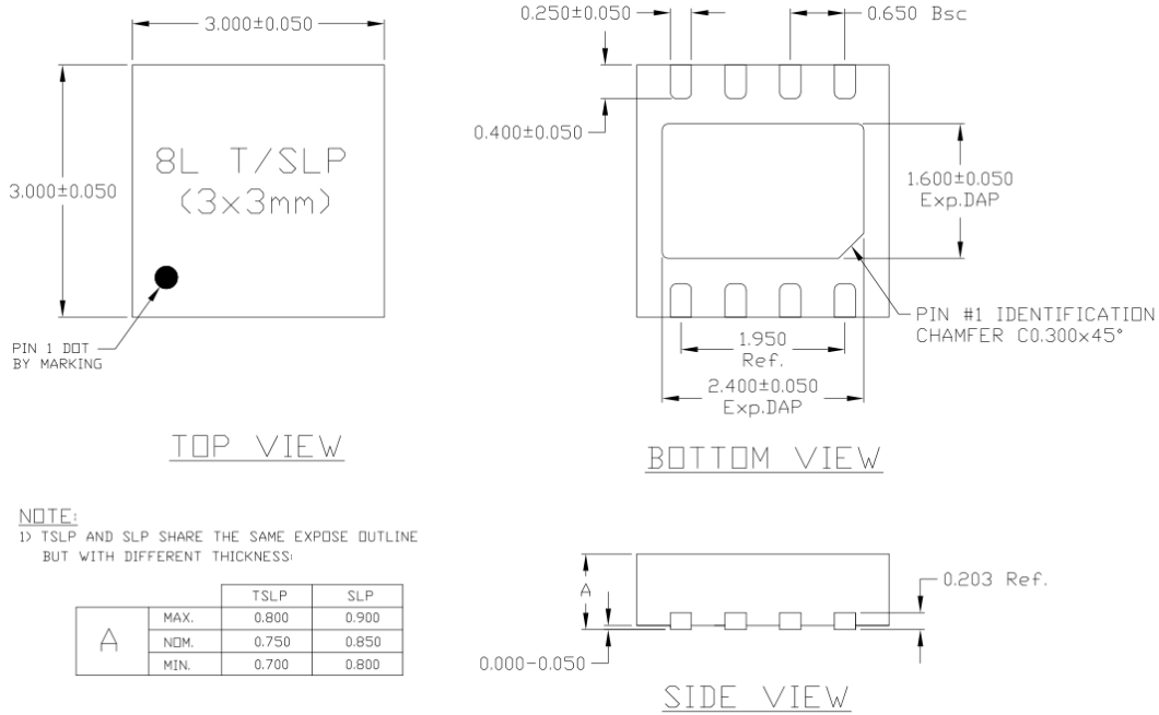
DFN3X3-8L Package Outline Dimensions
