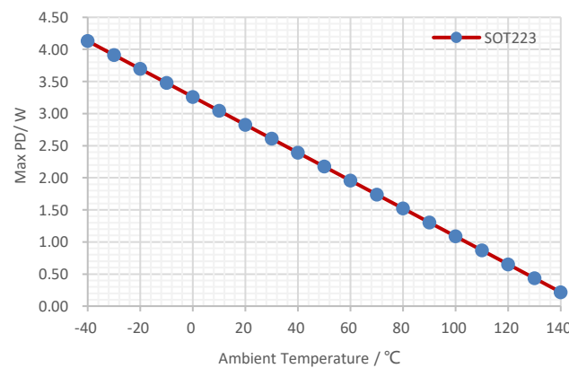
Figure 40. Maximum Allowed Power Dissipation vs Ambient Temperature, SOT223-4L, T_J \leq 150^\circ\text{C}
