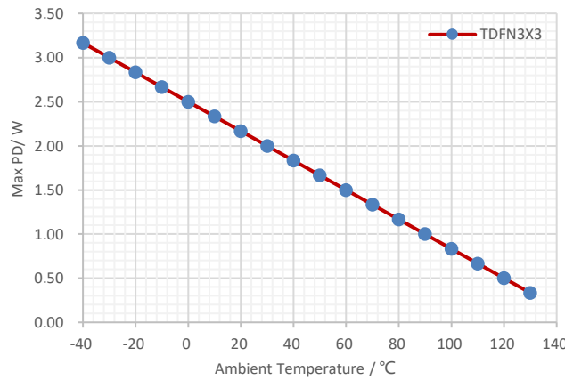
Figure 38. Maximum Allowed Power Dissipation vs Ambient Temperature, DFN3X3-8L, T_J \leq 150^\circ\text{C}
