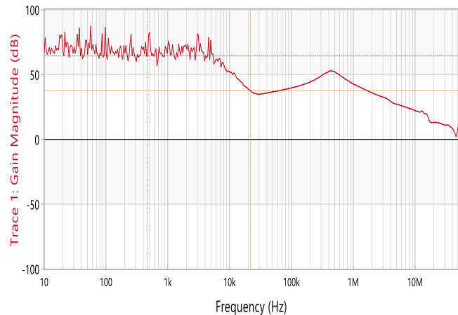
Figure 18. PSRR vs Frequency at Iout=100mA, C OUT =22uF
