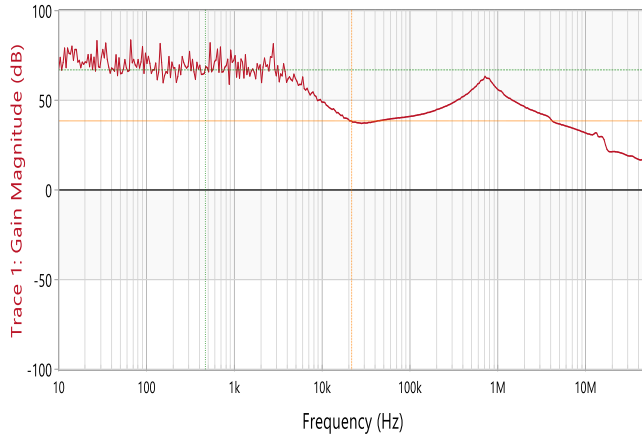
Figure 13. PSRR vs Frequency at Iout=10mA, C OUT =4.7uF
