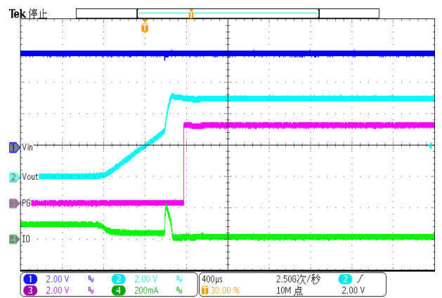
Figure 57. Exit Short Circuit Protection
