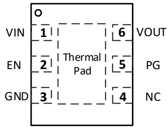
SCT71403FxxAQDVAR DFN2X2-6L Package
