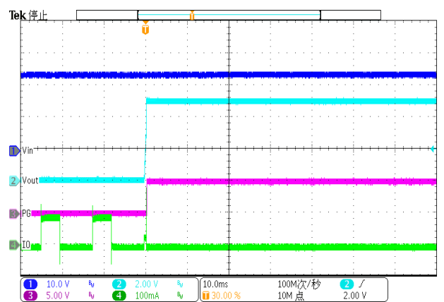
Figure 59. Exit Over Temperature Protection
