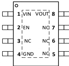
SCT71403FxxQMTER EMSOP-8L Package
