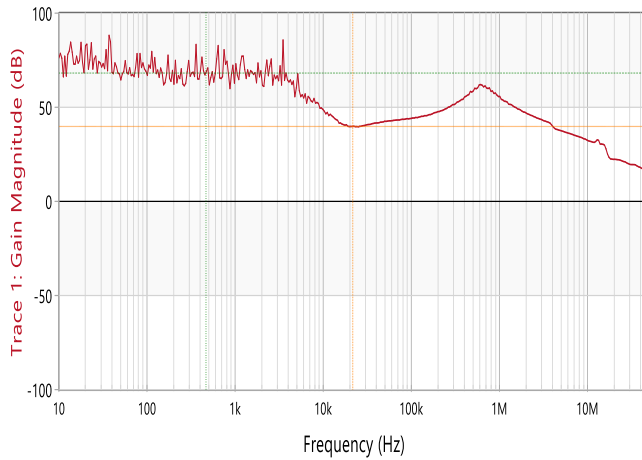
Figure 15. PSRR vs Frequency at Iout=10mA, C OUT =10uF
