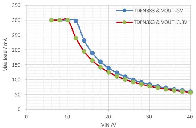
Figure 39. Maximum Output Current vs Input Voltage, DFN3X3-8L, T_J \leq 150^\circ\text{C}
