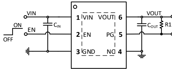
Figure 26. SCT71403Q Typical Application Schematic
