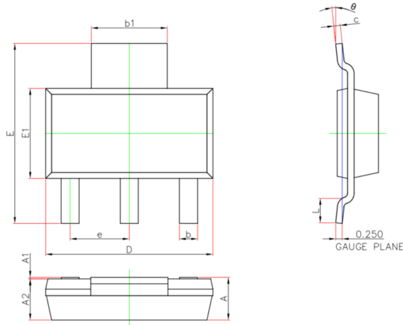
SOT223-4L Package Outline Dimensions
