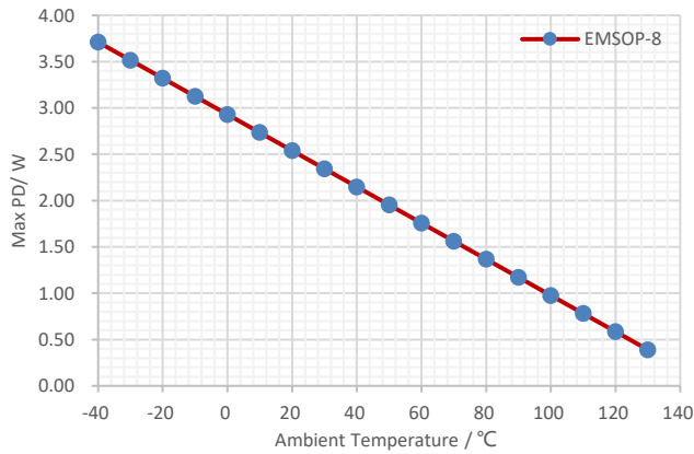
Figure 36. Maximum Allowed Power Dissipation vs Ambient Temperature, EMSOP-8L, T_J \leq 150^\circ\text{C}
