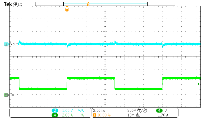
Figure 20. Load Transient (0.875A-2.625A, 1.6A/us)
