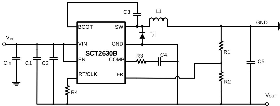
Figure 12. SCT2630B Inverting Power Supply
