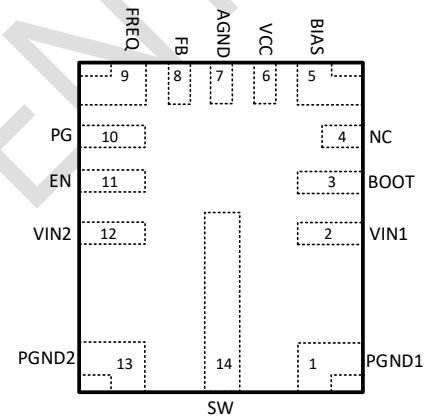
Figure1. 14-Lead FCQFN 4mm×4mm (Sketch Map)
