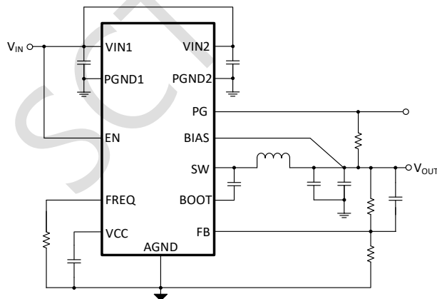
3.5V-36V, Synchronous Buck Converter
