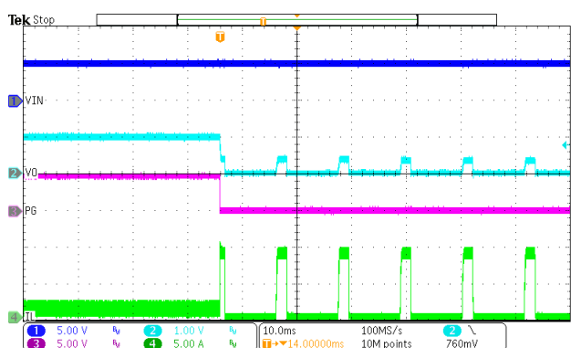
Figure 15. Over Current Protection(1A to hard short) ILIMIT=7A
