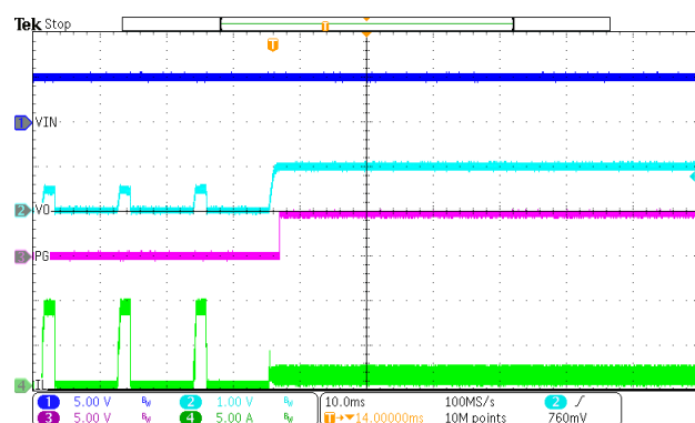
Figure 16. Over Current Release (hard short to 1A) ILIMIT=7A
