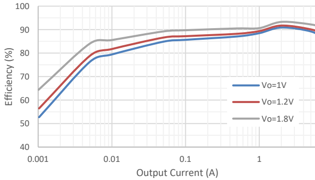
Figure 2. Efficiency at VIN=5V, Fsw=800kHz, PFM mode
