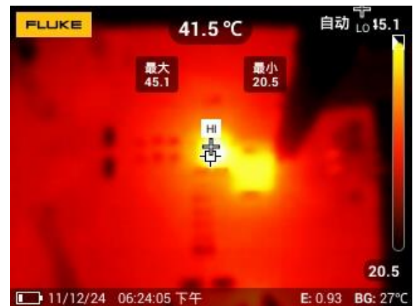
Figure 22. Thermal, Fsw=800kHz, Iload=6A
