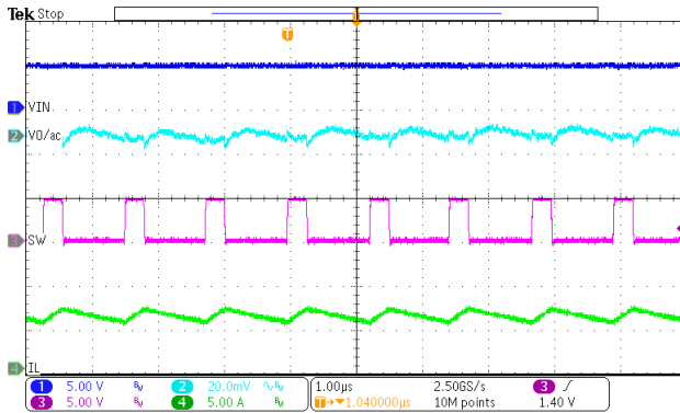
Figure 19. Output Ripple (Iload=6A, Fsw=800kHz)
