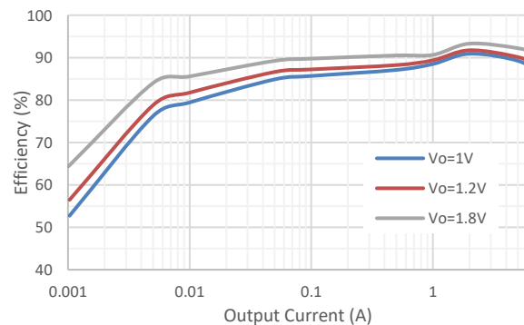
Vin=5V, fsw=800kHz, PFM Mode
