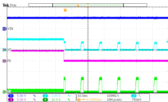
Figure 15. Over Current Protection(1A to hard short) ILIMIT=14A
