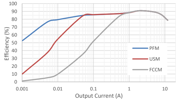
Figure 3. Efficiency at VIN=5V, Vout=1V, Fsw=800kHz
