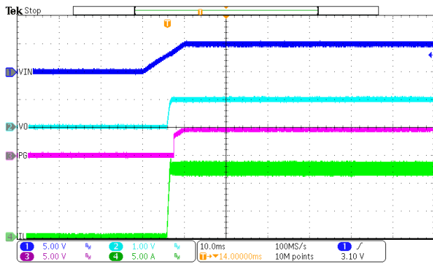
Figure 11. Power up (Iload=12A)
