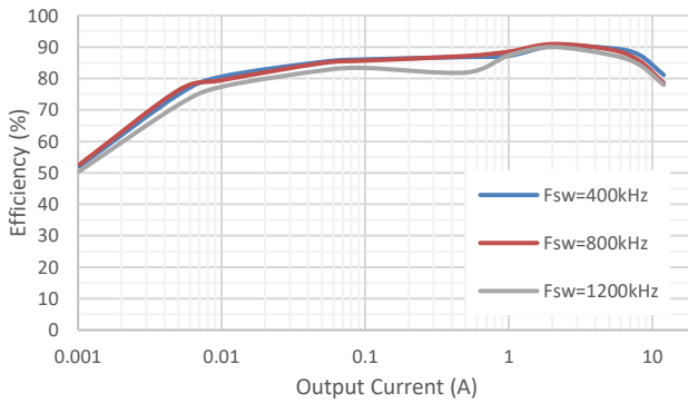
Figure 4. Efficiency at VIN=5V, Vout=1V
