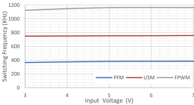
Figure 6. Switching Frequency VS Input Voltage
