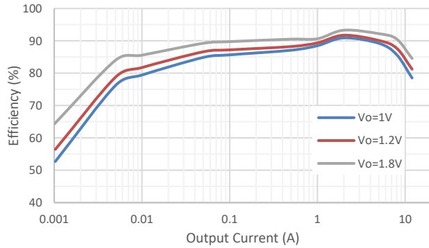
Figure 2. Efficiency at VIN=5V, Fsw=800kHz, PFM mode
