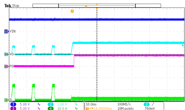
Figure 16. Over Current Release (hard short to 1A) ILIMIT=14A
