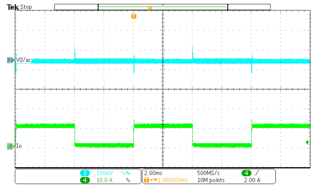
Figure 20. Load Transient (0A-10A, 1.6A/us)
