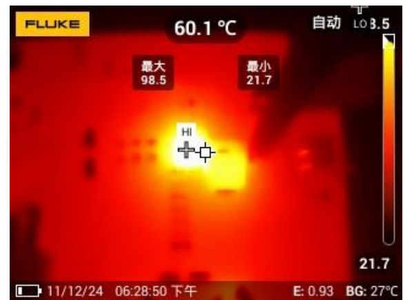
Figure 22. Thermal, Fsw=800kHz, Iload=12A
