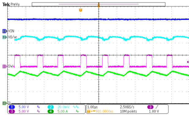
Figure 19. Output Ripple (Iload=12A, 800kHz)
