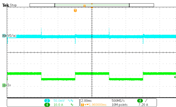
Figure 21. Load Transient (5A-10A, 1.6A/us)
