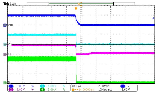
Figure 12. Power down (Iload=12A)
