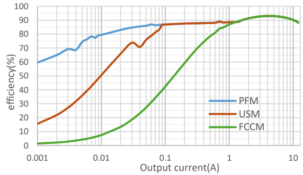
Figure 2. Efficiency VIN=12V, Vout=1.8V, Fsw=400kHz
