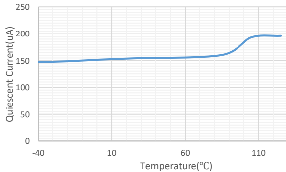
Figure 5. Quiescent Current VS Temperature
