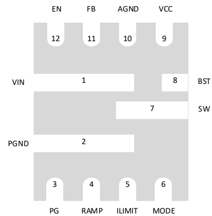
Figure 1. 12-Lead Plastic FCTQFN ( Top view: 2mmx3mm)
