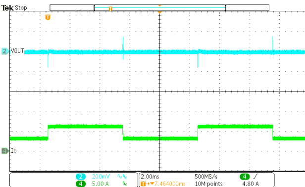
Figure 21. Load Transient (3A-6A, 1.6A/us)
