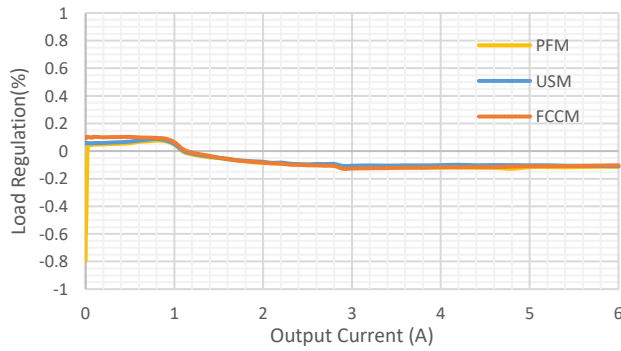
Figure 4. Load Regulation
