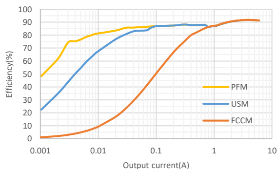
VIN=12V, Vout=3.3V, fsw=2.2MHz
