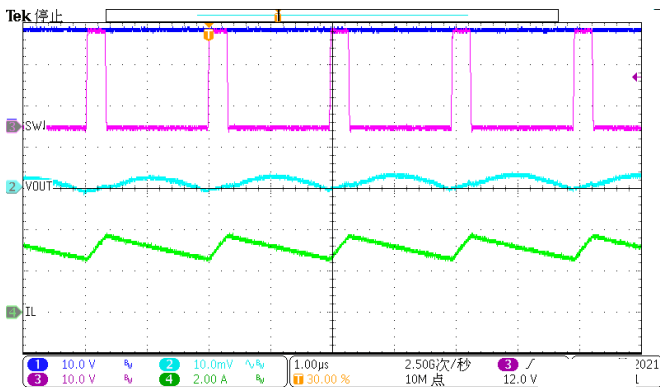
Figure 24. Output Ripple (Iload=3A)
