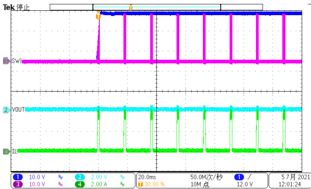
Figure 18. Over Current Protection (poweron to hard short)
