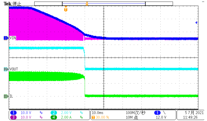
Figure 15. Power down
