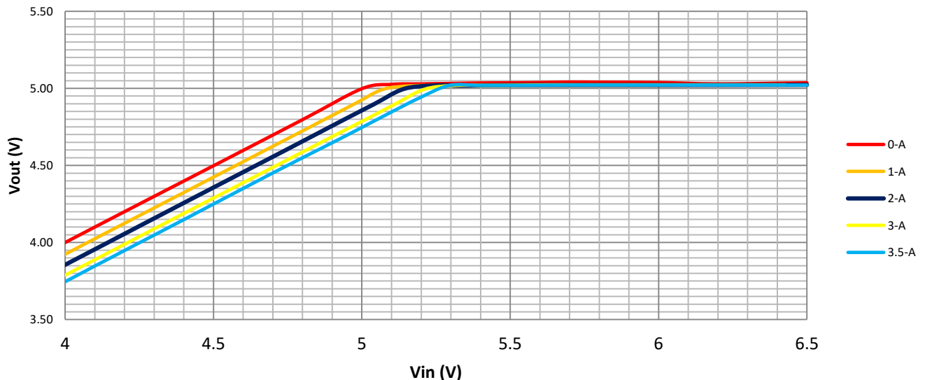
Figure 11. LDO Operation Characteristic ( Vout =5V )
