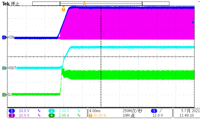
Figure 14. Power up
