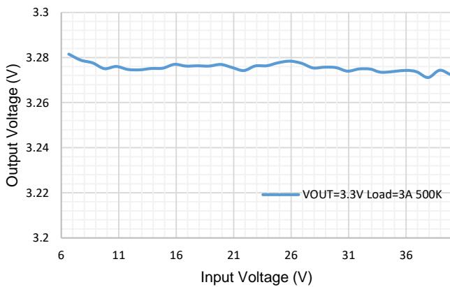
Figure 6. Line Regulation (IOUT=3A)
