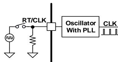
Figure 10. Setting Frequency and Clock Synchronization
