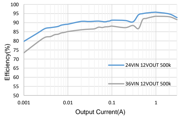
Figure 3. Efficiency vs Load Current, VOUT=12V, 500KHz
