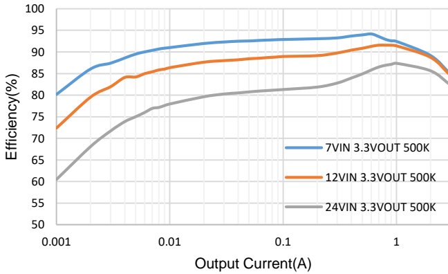
Figure 2. Efficiency vs Load Current, VOUT=3.3V, 500KHz
