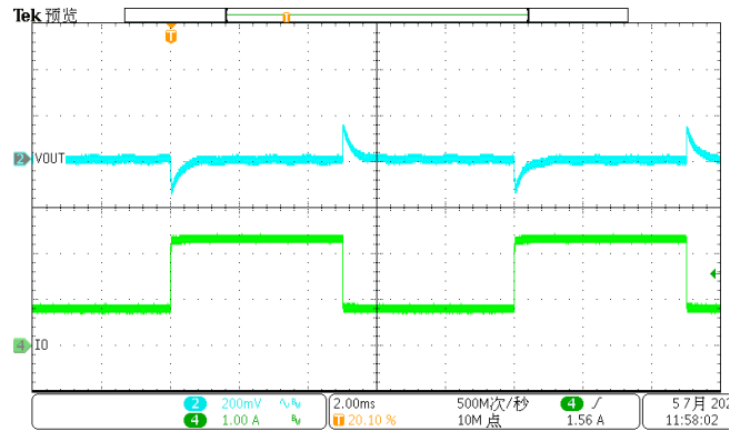
Figure 21. Load Transient (0.75A-2.25A, 1.6A/us)
