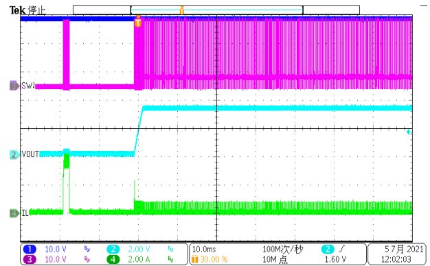
Figure 19. Over Current Release (hard short to 1A)
