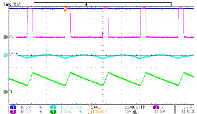
Figure 23. Output Ripple (Iload=1A)
