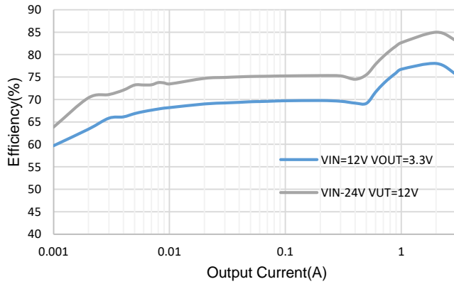
Figure 4. Efficiency vs Load Current, 2MHz
