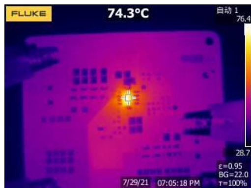
Figure 25. Thermal, 3.3Vout/3A
