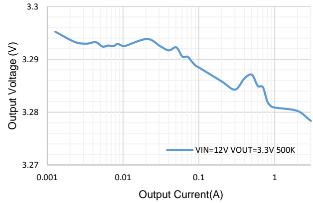
Figure 5. Load Regulation (VIN=12V, VOUT=3.3V)
