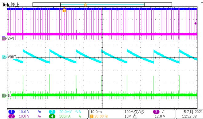
Figure 22. Output Ripple (Iload=0A)
