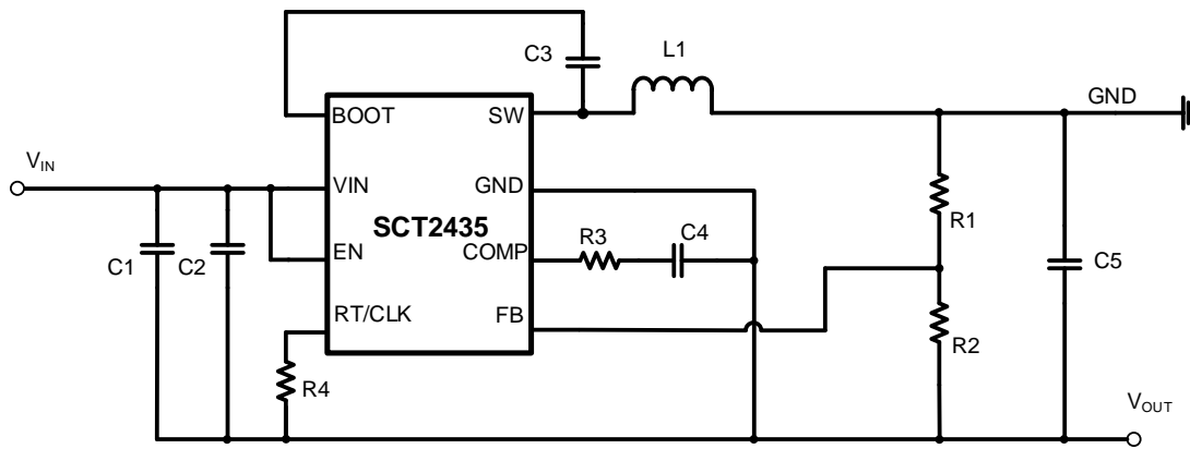
Figure 13. SCT2435 Inverting Power Supply
