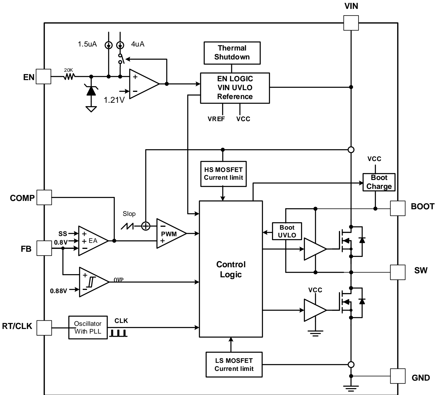
Figure 8. Functional Block Diagram
