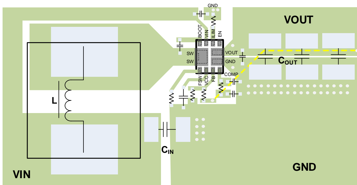
Figure 21. PCB Layout Example Top Layer
