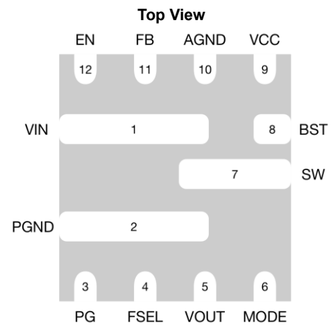
Figure 1. 12-Lead Plastic QFN (2mm×3mm)
